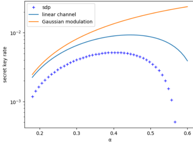
Figure 5.4: secret key rate vs \alpha , for a distance of 50 km and excess noise of \xi = 0.002 . Other parameters are the same as in Fig. 5.2
