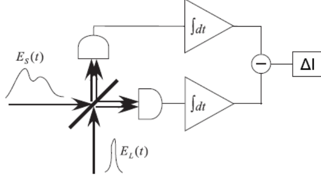
Figure 2.2: Homodyne detection setup (from Ref [14]).
