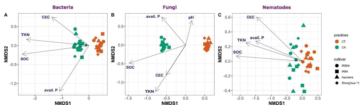
Sup. figure 7. Soil variables projected on the NMDSs of the communities of bacteria ( A ), fungi ( B ) and nematodes ( C ) with the function envfit of the package vegan . Only significant variables: pH, available phosphorus (avail. P), total Kjeldahl nitrogen (TKN), soil organic carbon (SOC) and cation exchange capacity (CEC). Stressplot = 0.10 ( A ), 0.080 ( B ) and 0.20 ( C ).
