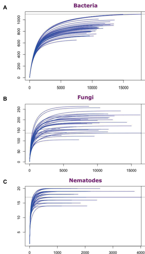
Sup. figure 6. Rarefaction curves for the communities of bacteria ( A ) and fungi ( B ): number of ESVs = f(\text{total reads count}) , or for the community of nematodes ( C ): number of families = f(\text{total individuals count}) .
