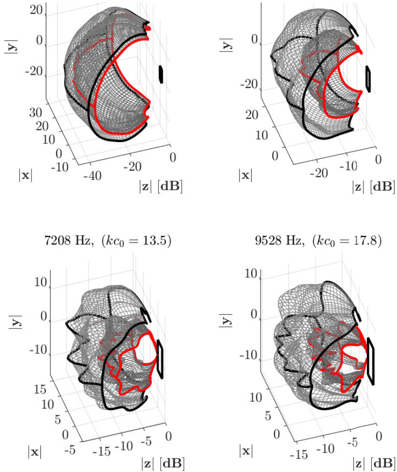
Figure 3.14: Experimental three-dimensional directivity plots corresponding to both baseline (black) and serrated flat-plate (red) of h/c_0 = 0.1 at Mach number M = 0.09 . Results are presented at Helmholtz numbers of kc_0 = 2, 7.5, 13.5 and 17.8 . The flow is delivered from negative to positive values along the x axis.
