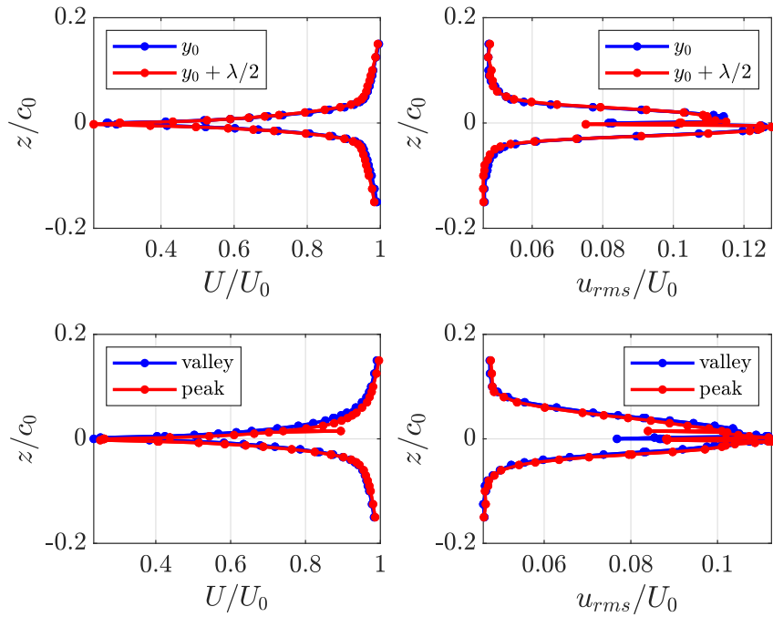
Figure 3.36: Mean velocity profiles U_0 (left) and u_{rms} (right) measured at the wake downstream at the very vicinity of the trailing edge of the baseline NACA12 (top) and the correspondent serrated (down). The two positions correspond to the serration valley and the serration peak. U_0 = 20 m/s.
