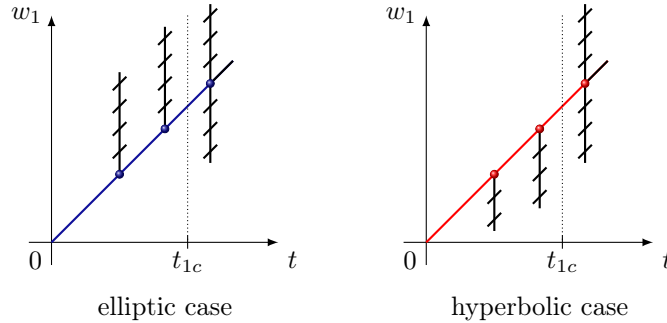
FIGURE 7.1 – Projection of the fixed time accessibility set on the w_1 -coordinate.
