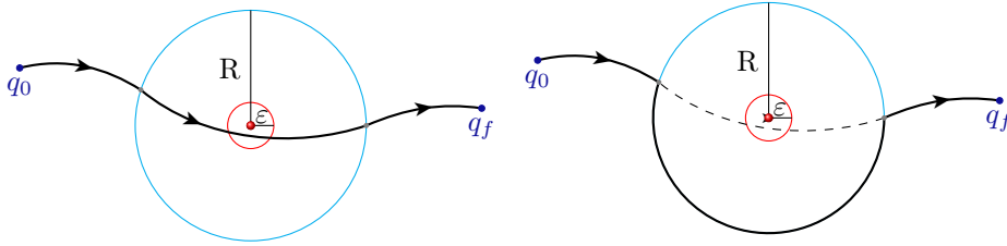
FIGURE 8.10 – Illustration of the construction of a strictly better admissible trajectory. The vortex is represented by a red ball, while the trajectories are the solid black lines. One can see on the left, a trajectory crossing the ball of radius \varepsilon . This trajectory is replaced on the right sub-graph by a strictly better admissible trajectory.
