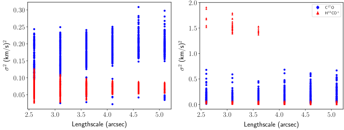
Figure 4.18: Values of \sigma^2 for each pixel in the analyzed region, for \text{C}^{17}\text{O} and \text{H}^{13}\text{CO}^+ , and for the blue- (left) and red-shifted (right) velocity components.
