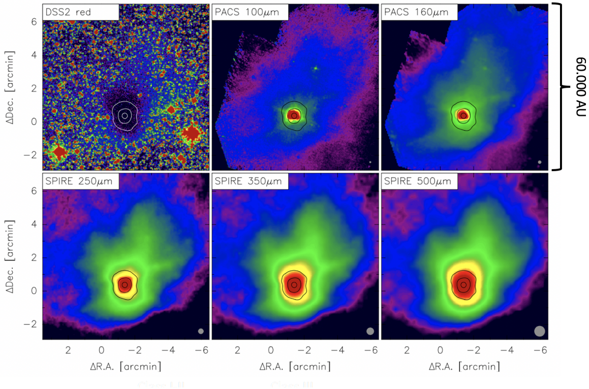
Figure 1.15: B335: Digitized Sky Survey 2 (DDS2) and Herschel FIR maps (color; log scale) at 100, 160, 250, 350 and 500 \mu\text{m} with 850 \mu\text{m} contours overlaid (100, 300 and 900 \text{mJy}/20'' beam). The Herschel beam is shown in gray (Launhardt et al. 2013). The scale is shown on the right considering a distance of 164.5 pc.
