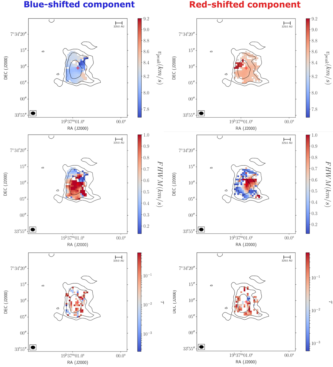
Fig. 5. C 17 O (1–0) maps obtained from modeling the line profiles with two velocity components. Overlaid contours show the integrated intensity at 5, 10, 20 and 30 \sigma , where \sigma is 10.0 mJy beam -1 . Top : peak velocity. Middle : linewidth. Bottom : opacity. Each column shows one of the two velocity components. Red crosses indicate the centroid position of B335.
