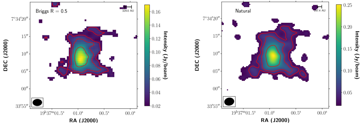
Figure 3.3: Integrated intensity images of \text{C}^{17}\text{O} (1-0) using different imaging parameters. Both images have been obtained by integrating in a velocity range 4.8-6.2 and 7.6-9.4 \text{km s}^{-1} accounting for the hyperfine structure of the line. Contours show integrated intensity at -3, 3, 5, 10 and 30 \sigma . Left : Briggs weighting with Robust parameter of 0.5 where \sigma = 10.6 mJy/beam (Map #6). Right : Natural weighting where \sigma = 13.4 mJy/beam (Map #7).
