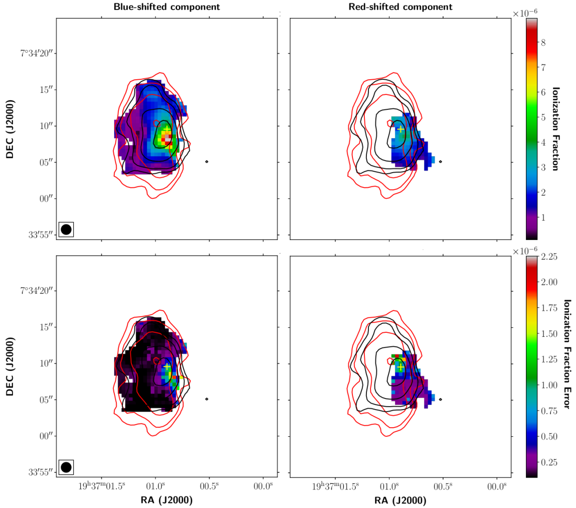
Figure 4.16: In contours, \text{DCO}^+ (3-2), in red, and \text{H}^{13}\text{CO}^+ (3-2) emission, in black, at 3, 5, 10 and 30\sigma (values of \sigma for each molecule are indicated in Table 4.1). In intensity scale, ionization fraction maps (top) and ionization fraction error (bottom), both in arbitrary units, for the blue- (left) and red-shifted (right) velocity components. The yellow cross indicates the centroid position of the source.
