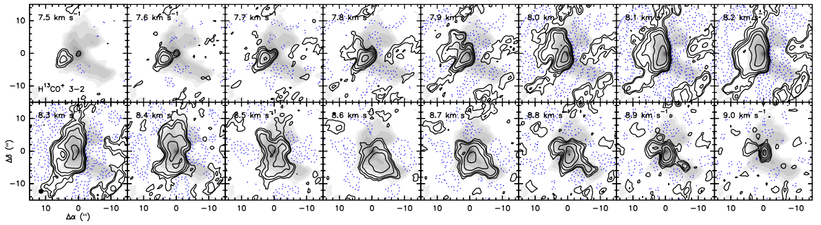
Figure 4.9: Same as Fig. 4.8 for \text{H}^{13}\text{CO}^+ (3-2).
