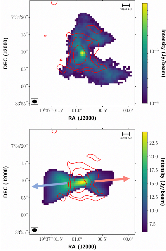
Fig. 1. Red contours showing moment 0 of \text{C}^{17}\text{O} emission, integrated over the velocity range 4.8\text{--}6.2\text{ km s}^{-1} and 7.6\text{--}9.4\text{ km s}^{-1} . Contours show emission at -3, 3, 5, 10 and 30\sigma , where \sigma is 10.0\text{ mJy beam}^{-1} . Top: intensity shows dust continuum emission map at 110\text{ GHz} for emission over 3\sigma , where \sigma is 8.56 \times 10^{-2}\text{ mJy beam}^{-1} . Bottom: intensity shows ^{12}\text{CO} (2–1) moment 0 emission integrated over the velocity range 1.4\text{--}16.2\text{ km s}^{-1} , for emission over 3\sigma , where \sigma is 2016.9\text{ mJy beam}^{-1} . The two arrows show the direction of the E-W outflow.
