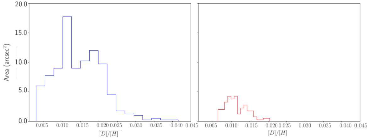
Figure 4.15: Histograms for the values of the deuteration fraction for the blue- (left) and red-shifted (right) velocity components.
