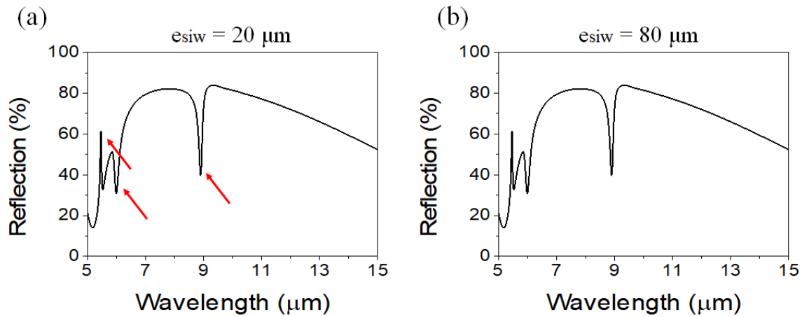
Figure 2.4: Reflection spectra of PolySi / Air / Si structure ( h = 750 nm, L = 4 \mu\text{m} , P = 5 \mu\text{m} , e_{air} = 2 \mu\text{m} ) for a non-polarized incident for a substrate silicon thickness (a) e_{siw} = 20 \mu\text{m} , and (b) e_{siw} = 80 \mu\text{m} .
