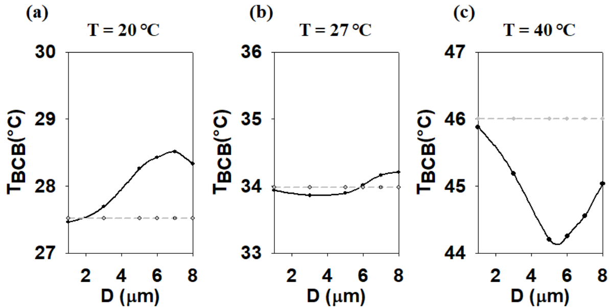
Figure 3.21: Evolution of the temperature of the membrane T_{BCB} , as a function of the holes diameter for a structured (solid lines) with P = 10 \mu\text{m} , h = 5.7 \mu\text{m} and non-structured (dashed lines) membrane at three different room temperatures: (a) T_{amb} = 20 \text{ }^\circ\text{C} , (b) T_{amb} = 27 \text{ }^\circ\text{C} , and (c) T_{amb} = 40 \text{ }^\circ\text{C} .
