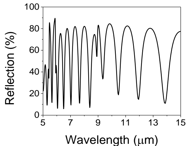
Figure 2.5: Reflection spectrum of a normally incident non-polarized light for the reference system of PolySi / Air / Si structure ( h = 750 nm, L = 4 \mu\text{m} , P = 5 \mu\text{m} , e_{siw} = 20 \mu\text{m} ) with e_{air} = 42 \mu\text{m} .
