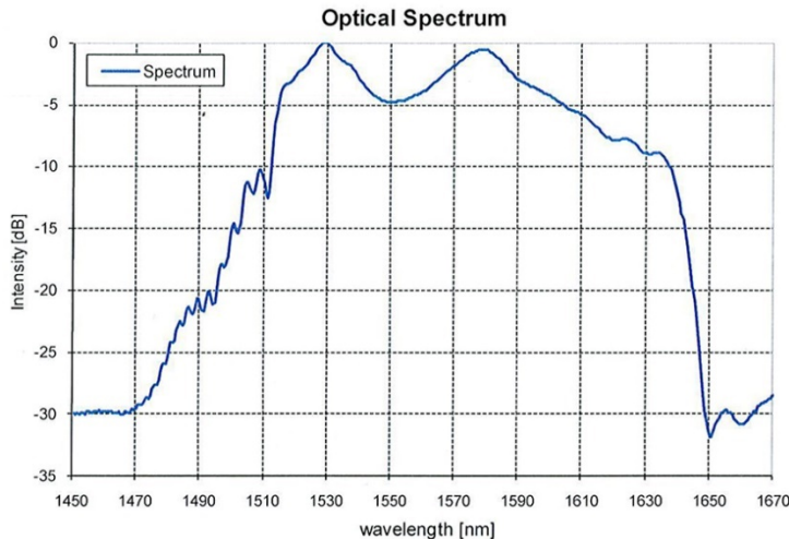
Figure 2-24 Optical spectrum of the Menlo femtosecond laser. Source: datasheet of the laser [69]
