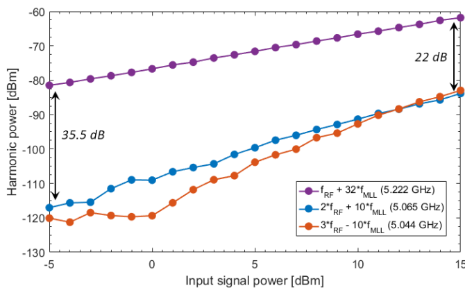
Figure 4-33 Power levels of selected harmonics of the mixing products at the switch output. f_{RF} = 2.022 GHz, P_{RF} = 15 dBm
