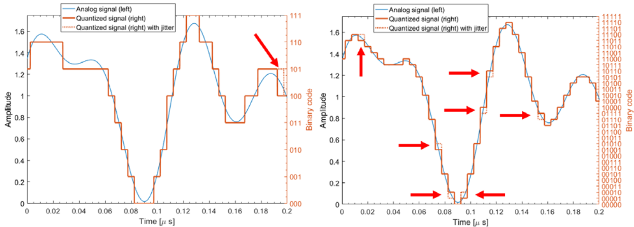
Figure 1-26 Illustration of the jitter effect on the quantized signal for 3 bits (left) and 5 bits (right), sampling rate is 200 MHz.
