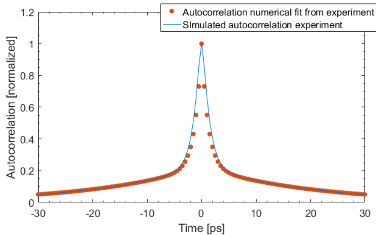
Figure 6 Simulated autocorrelation experiment (M) and numerical fit from the experiment (A) (see Figure 2-37).
