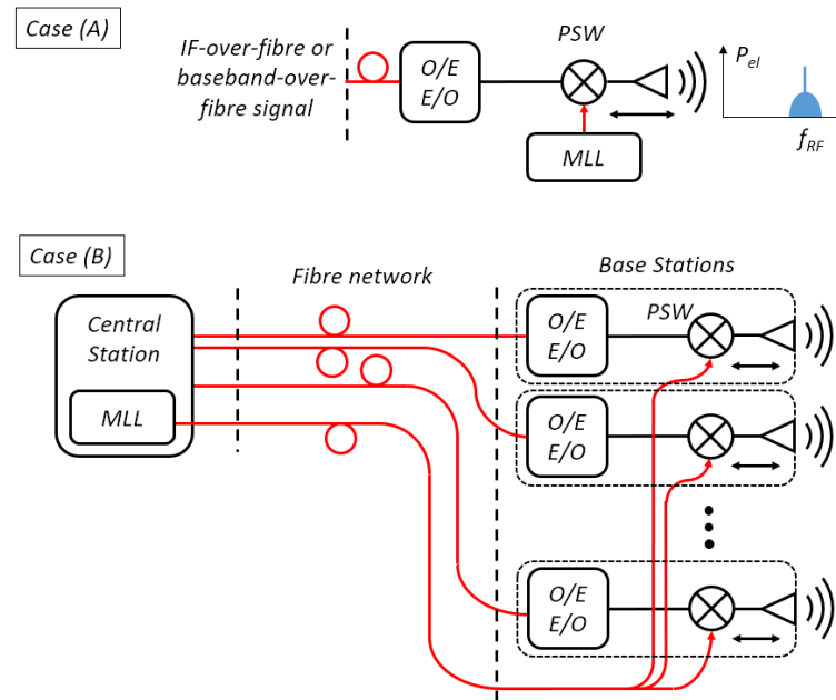
Figure 4-36 Concepts of the photoconductive switch use in RoF networks. O/E: optical to electrical converter; E/O: Electrical to optical converter; PSW: photoconductive switch
