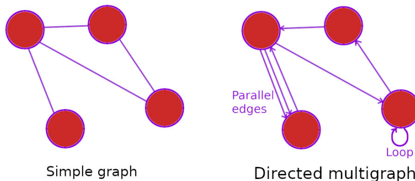
Figure 2.2: An example of a simple graph on the left, which contains non-weighted, undirected edges, no loops, and no parallel edges. On the right, an example of a directed multigraph, with non-weighted, directed edges, one loop, and multiple (parallel) edges.
