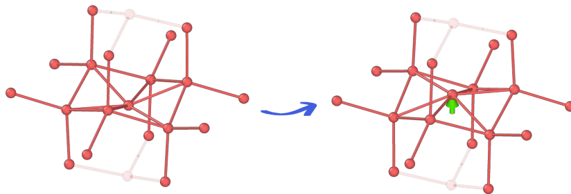
Figure 5.19: Hexagonal to hexagonal outside . The interstitial atom diffuses to neighbouring hexagon of the diamond structure.
