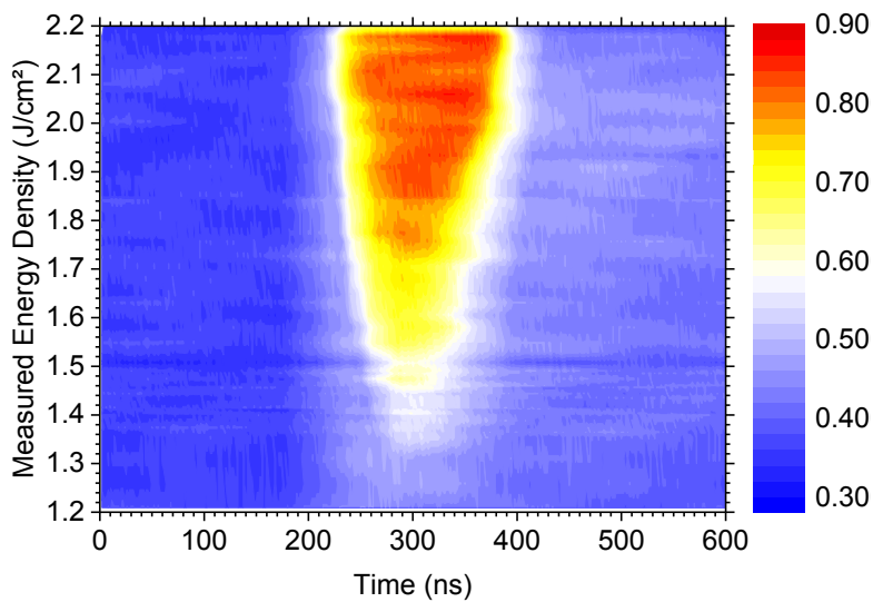
Figure III - 2. TRR colormap illustrating the evolution of the TRR signal as a function of time and laser energy density between 1.20 and 2.20 \text{J}/\text{cm}^2 , for a 30 nm-thick \text{Si}_{0.6}\text{Ge}_{0.4} layer submitted to UV-NLA. The melt threshold is found close to 1.35 \text{J}/\text{cm}^2 . The maximum energy density step was 50 \text{mJ}/\text{cm}^2 , and was as low as 10 \text{mJ}/\text{m}^2 near the melt threshold to study the transition.
