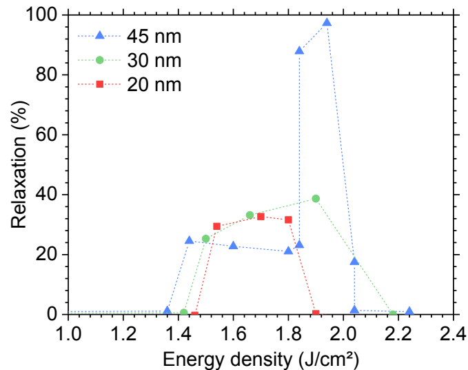
Figure IV - 13. Evolution of the macroscopic strain relaxation level as a function of laser energy density for 20, 30 and 45 nm-thick Si 0.7 Ge 0.3 layers. Some plots exhibit two relaxation values for a given energy density: it is caused by the appearance of two SiGe peaks in the RSM.
