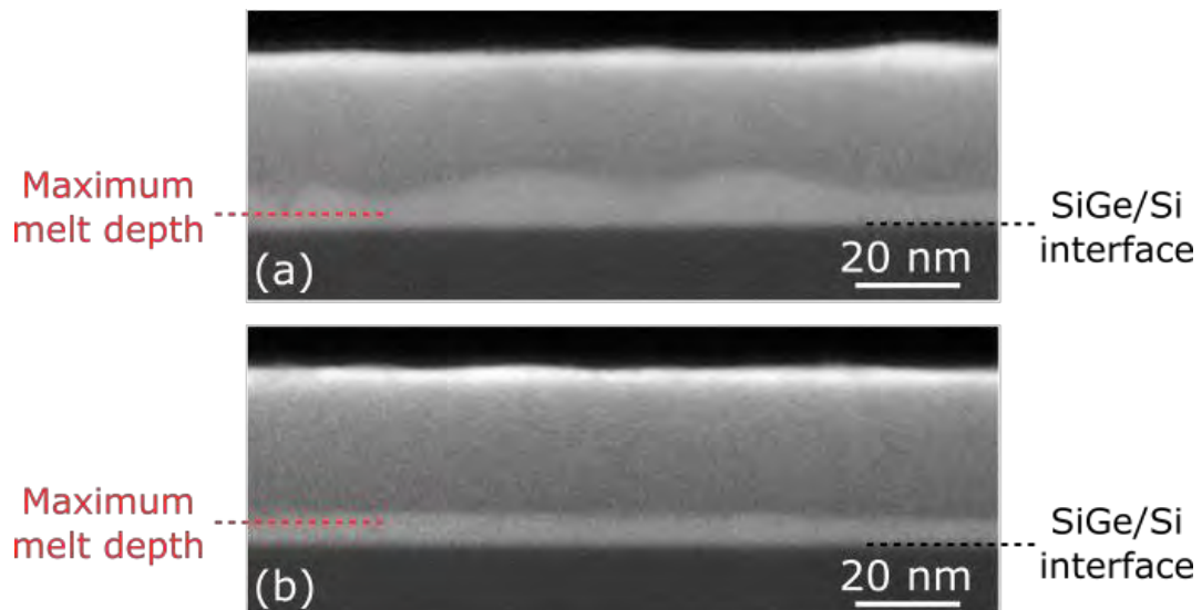
Figure IV - 25. STEM-HAADF images on \text{Si}_{0.7}\text{Ge}_{0.3} samples annealed at 1.95 \text{ J/cm}^2 for sample A (a) and sample C (b).
