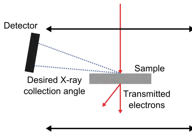
Figure II - 22. X-ray detection for EDX observations in TEM
