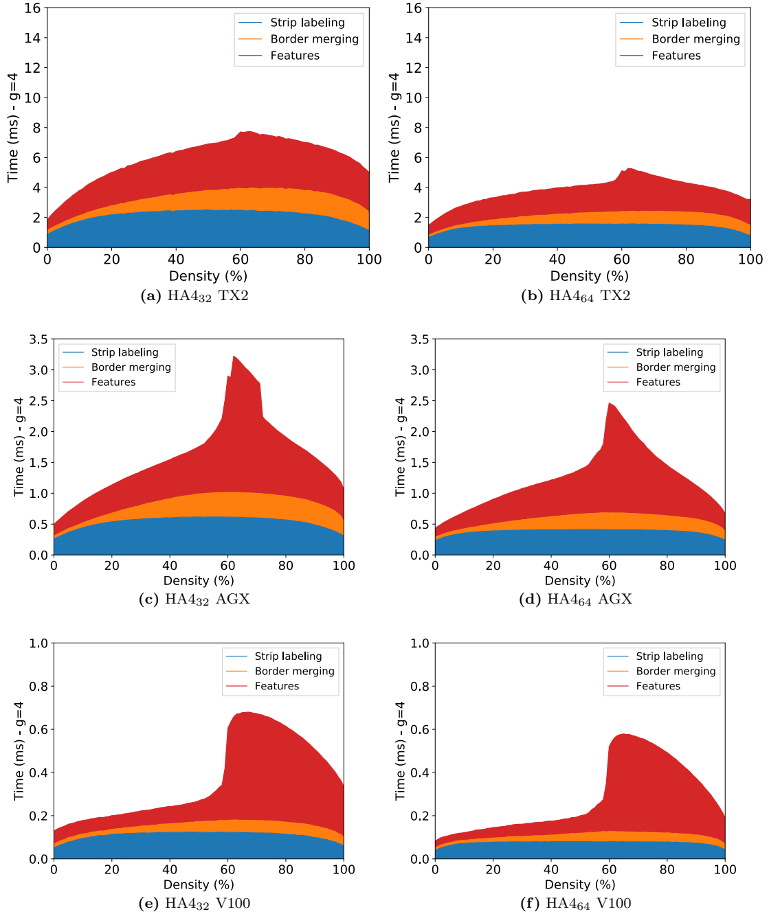
Figure 4.13: Analysis of the execution time for 2048 \times 2048 images, g = 4 .
