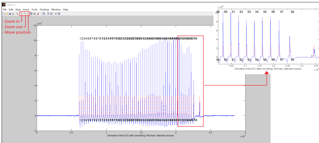
Figure 3.19: Two operations for f_0 dEGG verification. The example is taken from the data of speaker M1, first token 0101, target syllable /paj 5 / in isolation.
