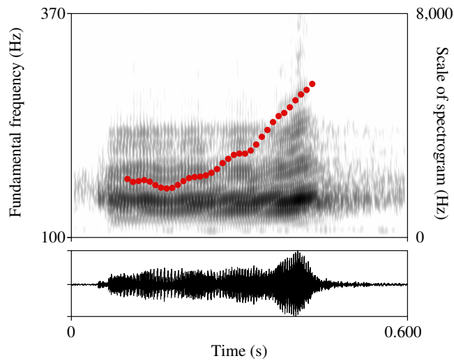
Figure 2.6: Vietnamese tone C1 ( hỏi ), as realized in isolation over the syllable / kɤ / by a speaker from Hanoi. Year of recording: 1900.
