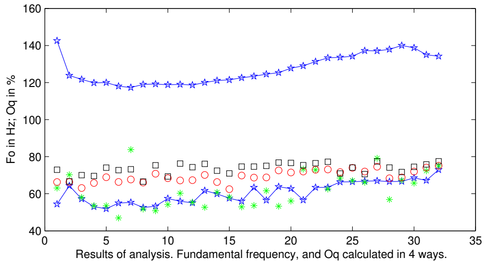
Figure 3.26: An example of O_q dEEG curves with large differences across methods as a result of imprecise opening peaks. Reproduced from M.-C. Nguyễn (2016): data of speaker M1, experiment 2, item 1331.
