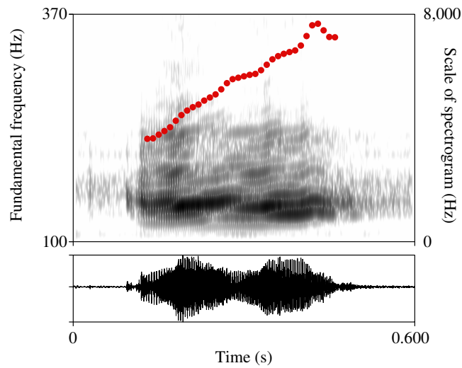
Figure 2.4: Vietnamese tone B1 ( sắc ), as realized in isolation over the syllable / kɤ / by a speaker from Hanoi. Year of recording: 1900.
