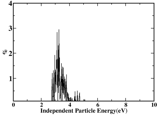
Figure 9.4: Transition plot for the excitonic peak
