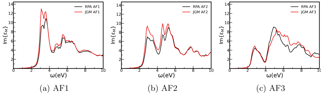
Figure 11.4: Linear response calculated using RPA and JGM kernel for three AFM structures of \text{Cr}_2\text{O}_3
