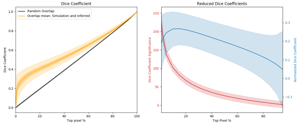
Figure 3.12: Left: dice coefficient (as defined by Eq. 3.3) of top n\% pixels between 2D simulation images and their inferred counterparts, by increments of 5% (yellow). The inner dark yellow layer represents measure uncertainty and the outer yellow layer represents standard deviation over the set. Random overlap is represented in black. Right, red: dice coefficient significance (see Eq. 3.5), blue: normalized dice coefficient (see Eq. 3.4); both are represented with their standard deviation layers.
