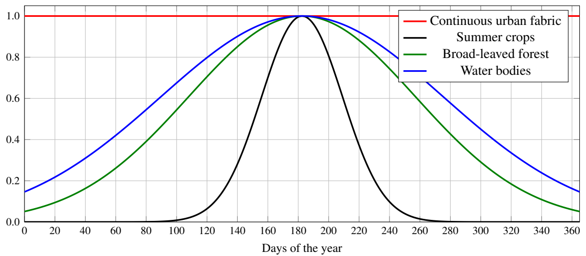
Figure 5.11: Normalized RBF kernels (5.8) centered at day 180: K(t, 180) = \exp(-0.5(t - 180)^2/h_c^2) computed on four classes.
