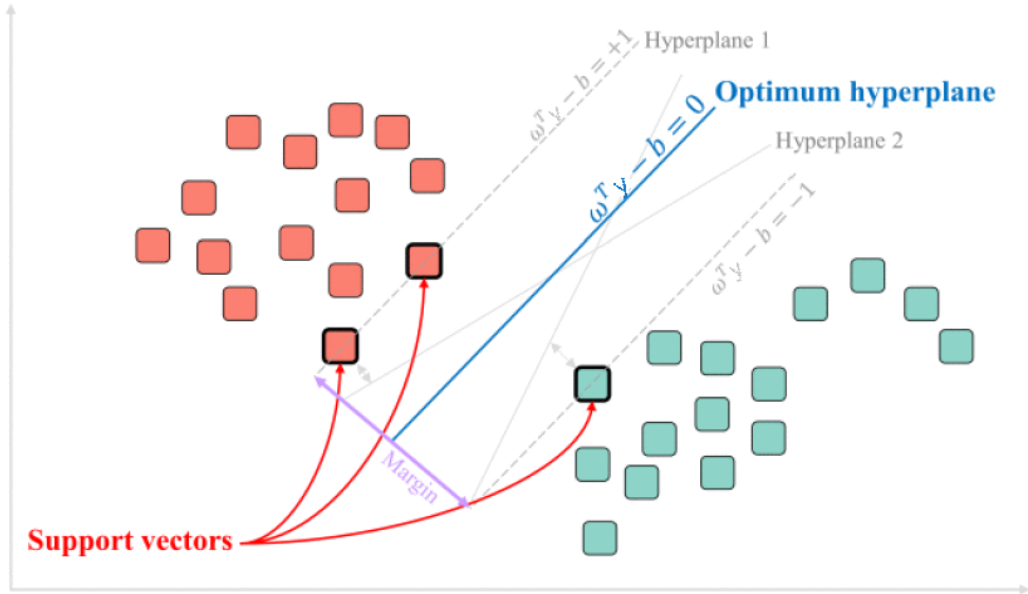
Figure 1.10: (Image from [160]). Two classes (red and green) are separated thanks to the optimal hyperplane (blue line), i.e. the hyperplane which maximizes the margin between the two groups. In this example the data \mathbf{y} are real-input vectors.
