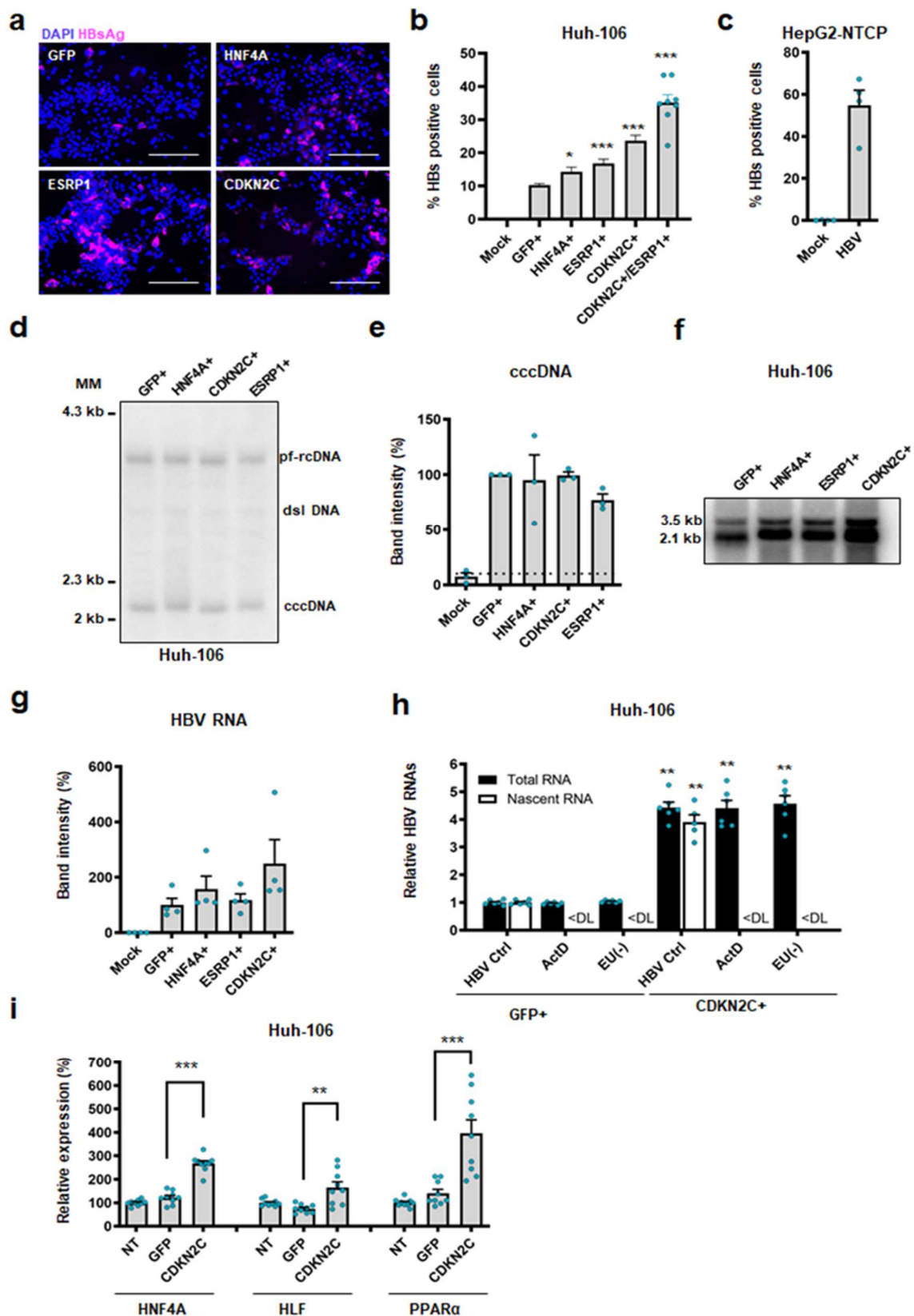
Figure 3.5. CDKN2C stimulates HBV cccDNA-mediated transcription. a-b, d-g Validation studies in Huh-106 overexpressing individual ORFs and infected with HBV for 10 days. a Detection of HBsAg by IF. Scale bars: 100 μm. b Flow-cytometric analysis for quantification of HBsAg-positive cells. Results are expressed as means \pm SEM % HBsAg positive cells compared to GFP from 5 independent experiments (n=13, n=11 for HNF4A) and 3 independent experiments (n=8) for CDKN2C+ESRP1. c Flow-cytometric analysis for quantification of HBsAg-positive cells in HBV-infected HepG2-NTCP cells. Results are expressed as means \pm SEM % HBsAg positive cells from 4 independent experiments (n=4). d-e Detection of HBV DNAs by Southern Blot in transduced and HBV infected Huh-106 4 dpi. d Southern Blot with indicated bands of HBV pf-rcDNA, dsI HBV DNA and HBV cccDNA. One representative experiment is shown.
