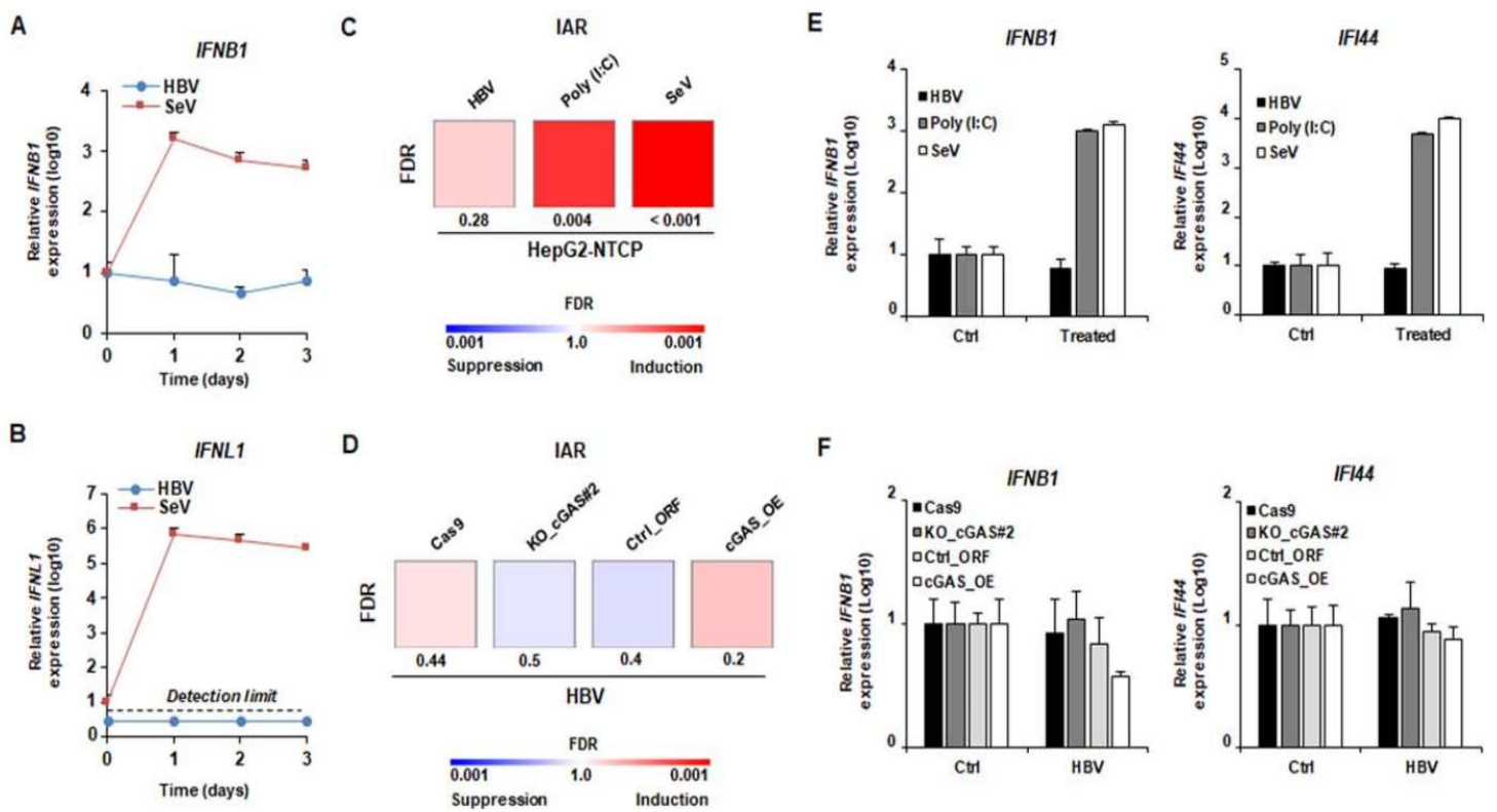
Figure 2. Impaired cGAS-mediated sensing of HBV infection in HepG2-NTCP cells. (A-B) HBV infection does not induce IFNB1 or IFNL1 expression. HepG2-NTCP cells were infected with HBV (MOI: 500) or SeV (MOI: 10) and total RNA was extracted every day for 3 days. RNA extracted from naive cells before infection was used as a control (D0). IFNB1 (A) and IFNL1 (B) expression was then assessed by qRT-PCR. Results are expressed as means \pm SD IFNB1/IFNL1 relative expression (log10) compared to controls (D0, all set at 1) from three independent experiments performed at least in duplicate (SeV) or four independent experiments performed in duplicate (HBV). No robust IFNL1 expression was detected in HBV-infected samples (representative dots are presented under the “detection limit” dotted line). (C, E) cGAS-related ISG are not affected by HBV infection. HepG2-NTCP cells were infected with HBV or SeV. Alternatively, HepG2-NTCP cells were transfected with Poly (I:C) (100ng). Two days after infection or transfection, total RNA was extracted. Gene expression of IAR signature was then analyzed using multiplexed gene profiling. Results were analyzed by GSEA enrichment compared to non-transfected or non-infected controls (C) or by IFNB1 and IFI44 gene expression (log10) compared to non-transfected or non-infected controls (set at 1) (E). One experiment performed in triplicate is shown. (D, F) cGAS expression level does not affect the cellular response to HBV infection. HepG2-NTCP-Cas9 (Cas9), HepG2-NTCP-KO_cGAS#2 (Ko_cGAS#2), HepG2-NTCP-Ctrl_ORF (Ctrl_ORF), and HepG2-NTCP-cGAS_OE (cGAS_OE) were infected with HBV. Two days after infection, total RNA was extracted. Gene expression of IAR signature gene set was then analyzed using multiplexed gene profiling. Results were analyzed by GSEA enrichment compared to non-transfected or non-infected controls (D) or by IFNB1 and IFI44 gene expression (log10) compared to non-transfected or non-infected controls (set at 1) (F). One experiment performed in triplicate is shown. IAR: innate antiviral response gene set.
