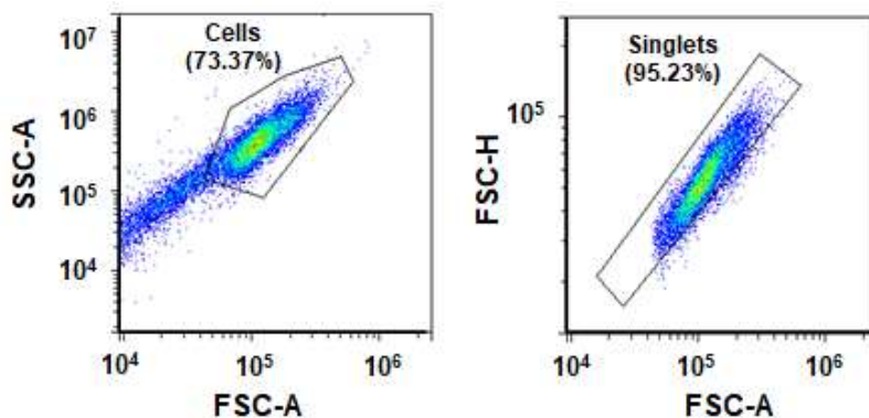
Figure S3.7 (related to Figures 2 and 7 ). Flow cytometry gating strategy using Huh-106 cells. The gating was performed using an FCS/SSC dot plot. The gain was adjusted when all cell populations were visible on the plot. The living cell population was gated to perform a “singlets” plot through FSC-H and FSC-A parameters. Histogram- and dot plots were obtained from the “singlets” gate using Count/APC-A or SSC-A/APC parameters.
