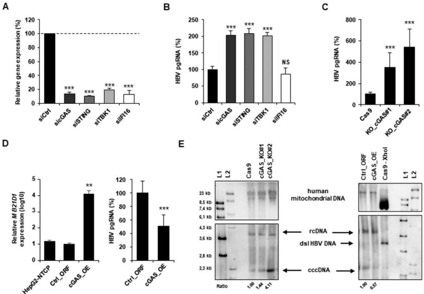
Figure 2.6. Antiviral activity of cGAS results in reduction of HBV cccDNA. (A-B) Silencing of cGAS-related gene expression increases HBV infection. siRNA targeting MB21D1 (sicGAS), TMEM173 (siSTING), TBK1 (siTBK1), IFI16 (siIFI16) or a non-targeting siRNA (siCtrl) were reverse-transfected into HepG2-NTCP cells 2 days prior to HBV infection. Silencing efficacy was assessed by qRT-PCR 2 days after transfection (A). Results are expressed as means \pm SD % gene expression relative to siCtrl (set at 100%) from four independent experiments performed in technical duplicate. HBV infection was assessed by quantification of HBV pgRNA by qRT-PCR 10 days after infection (B). Results are expressed as means \pm SD % HBV pgRNA expression relative to siCtrl (set at 100%) from four independent experiments performed in technical duplicate. (C) KO of MB21D1 gene increases HBV infection. cGAS_KO#1, cGAS_KO#2, and the control Cas9 cells were then infected with HBV and viral infection was assessed 10 days after infection as described above. Results are expressed as means \pm SD % HBV pgRNA expression relative to control cell line (Cas9, set at 100%) from three independent experiments performed in triplicate. (D) cGAS overexpression reduces HBV infection. HepG2-NTCP cells were transduced with lentivirus encoding either a control plasmid (Ctrl_ORF) or a plasmid encoding the full length MB21D1 ORF (cGAS_OE). MB21D1 expression was assessed by qRT-PCR (left panel). Results are expressed as means \pm SD % relative MB21D1 expression (log10) relative to control cell line (Ctrl_ORF, set at 1) from three independent experiments performed in duplicate. HepG2-NTCP, Ctrl_ORF, and cGAS_OE cells were then infected with HBV for ten days and HBV infection was assessed as described above. Results are expressed as means \pm SD % HBV pgRNA expression relative to control cell line (Ctrl_ORF, set at 100%) from three independent experiments performed in triplicate. (E) Detection of HBV cccDNA by Southern blot. HepG2-NTCP-derived cGAS_KO- or cGAS_overexpressing cell lines were infected for 10 days with HBV. Total DNA from indicated HBV infected cells was extracted and HBV DNA were detected by Southern blot. Two different DNA ladders (L1 & L2) were used. XhoI digestion of DNA extracted from HBV-infected HepG2-NTCP-Cas9 cells was used as a control and resulted in a single 3.2 kb band (dsI HBV DNA). Mitochondrial DNA (mt DNA) was detected as a loading control. One experiment is shown.
