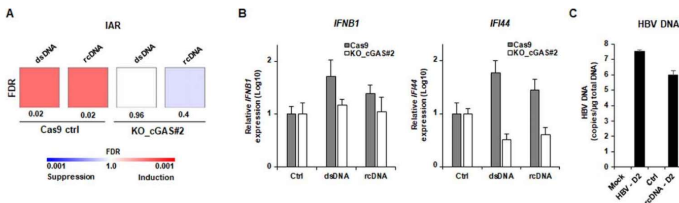
Figure 2.4. Sensing of HBV rcDNA in HepG2-NTCP cells. (A-B) Transfection of purified HBV rcDNA genome induces a cGAS-mediated innate immune response. HBV rcDNA was extracted from recombinant HBV virions as described in Experimental Procedures and quantified by qPCR (Figure S2.3). HBV rcDNA (1 μg) and positive control dsDNA (1 μg) were transfected into HepG2-NTCP-Cas9 and HepG2-NTCP-KO_cGAS#2 cells. Three days after transfection, total RNA was extracted. Gene expression of IAR set was then analyzed using multiplexed gene profiling. The transcripts were analyzed by GSEA enrichment compared to non-transfected control (A) or by IFNB1 and IFI44 gene expression (log10) compared to non-transfected control (set at 1) (B). One experiment in triplicate is shown. (C) HBV DNA in HepG2-NTCP cells after rcDNA transfection and HBV infection are similar. HepG2-NTCP were infected with HBV or transfected with HBV rcDNA (1μg). At day 2 after transfection/infection, DNA was extracted and total HBV DNA was quantified by qPCR. Results are expressed as means ± SD total DNA copies per μg of total DNA (log10) from three independent experiments performed in triplicate (HBV infection) and two independent experiments performed in triplicate (HBV rcDNA transfection). IAR: innate antiviral response gene set.
