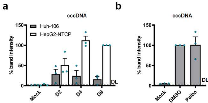
Figure S3.5. Quantification of Southern Blot cccDNA band using Image Lab Version 5.2.1 (related to (a) Figure 1e and (b) 7f ). a Quantification of cccDNA bands in Mock or HBV infected Huh-106 and HepG2-NTCP cells 2 (D2), 4 (D4) or 9 (Mock, D9) days post HBV infection. Results are expressed as means \pm SEM % band intensity compared to HBV-infected HepG2-NTCP D9 (set to 100%) from 3 independent experiments. Dashed line indicates the detection limit (DL). Related to Figure 1e. b Quantification of cccDNA bands in Mock or HBV infected Huh-106 cells treated with DMSO or 100 nM Palbociclib 4dpi. Results are expressed as means \pm SEM % band intensity compared to DMSO (set to 100%) from 3 independent experiments. Dashed line indicates the detection limit (DL). Related to Figure 7f . Source data are provided as a Source Data file.
