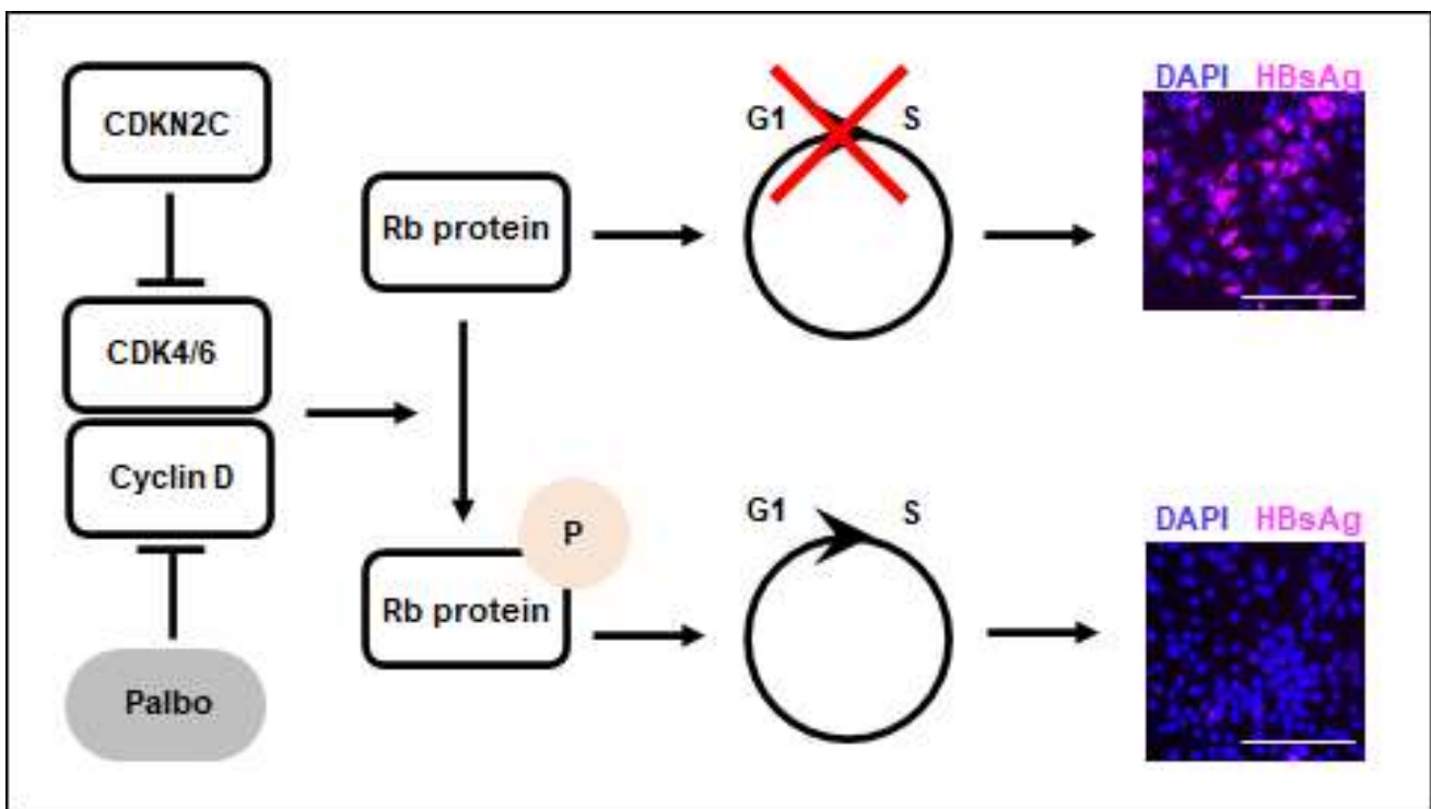
Figure 3.8. Schematic model of the effect of CDKN2C expression and Palbociclib (Palbo) treatment on HBV infection. CDKN2C and Palbociclib inhibit the CDK4/6 and Cyclin D mediated phosphorylation of Rb protein, leading to an accumulation of Rb protein in its unphosphorylated state. Unphosphorylated Rb protein induces a cell cycle G1 arrest resulting in increased HBV infection rates. Illustrative HBV infection pictures come from Fig. 6. Scale bars: 100 \mu m.
