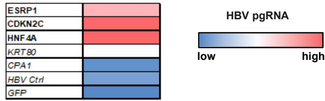
Figure 3.S1. Heatmap of candidate validation by quantification of pgRNA (related to Figure 3a ). Huh-106 cells were transduced with the indicated ORF and infected with HBV. HBV infection was assessed at 10 dpi by qRT-PCR quantification of pgRNA. Results are expressed as means relative pgRNA expression from 2 independent experiments (n=4).
