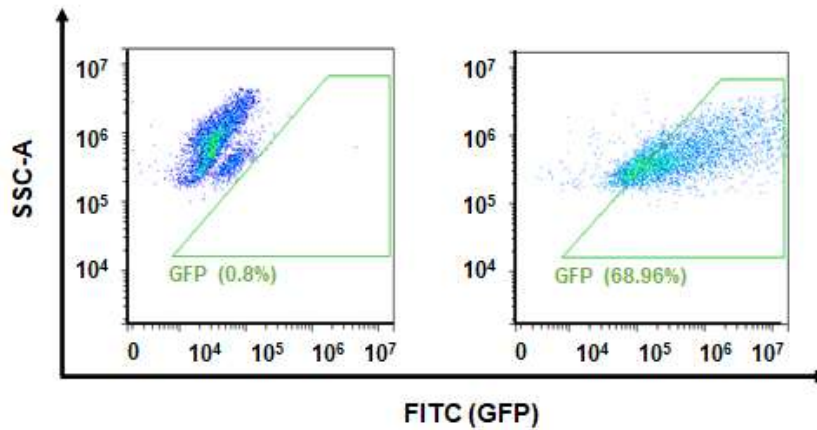
Figure 3.S2. GFP control vector (related to Figure 5b ). Expression of GFP in Huh-106 transduced with lentivirus for GFP overexpression (GFP) or non-transduced (NT). Quantification of GFP-expressing cell population by flow cytometric analysis in HBV-infected cells 10 dpi.
