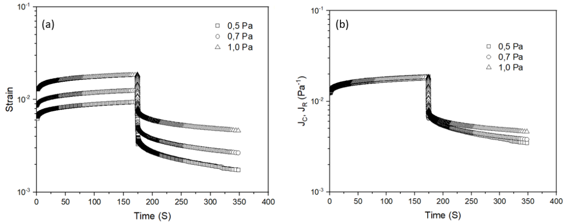
Fig. 3.14 Strain (a) and compliance (b) as a function of time, at the applied stresses \sigma = 0,5 , 0,7 and 1 Pa, for a 7 wt% Oht suspension.
