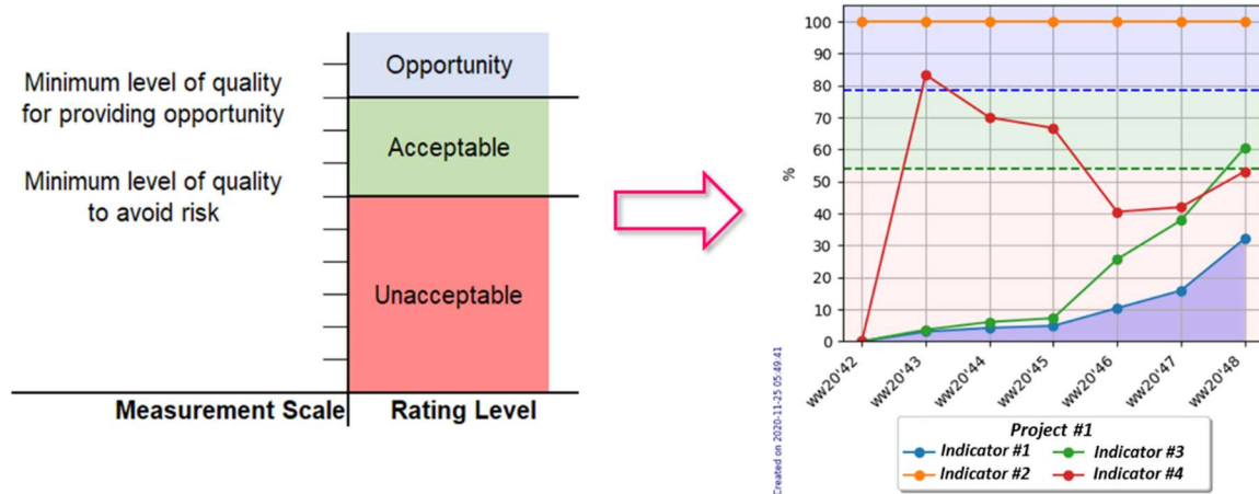
Figure 18 - Threshold for risk acceptance and opportunities: from ISO/IEC 25022 [140] theory to practice
