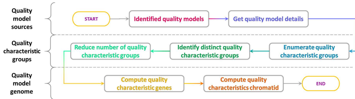
Figure 81 - The seven steps in the software quality model genome meta-model construction algorithm
