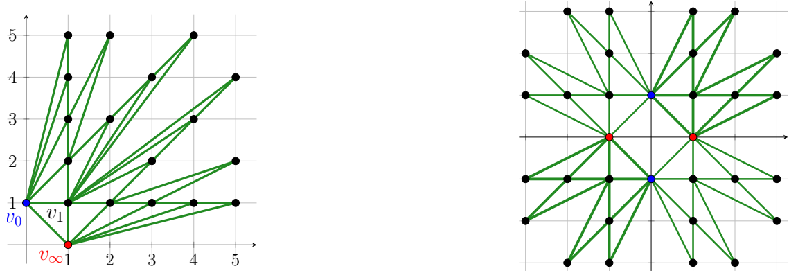
Figure 2.1: The lotus \Delta_1 and its quadruple \Delta_4 .
