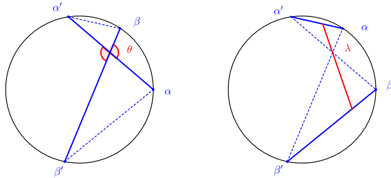
Figure 1.21: Cross-ratios and cosines in the real case.
