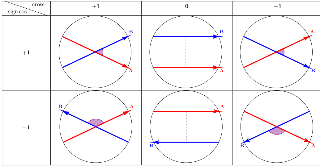
Figure 1.15: Drawing configurations: cross and sign cos.
