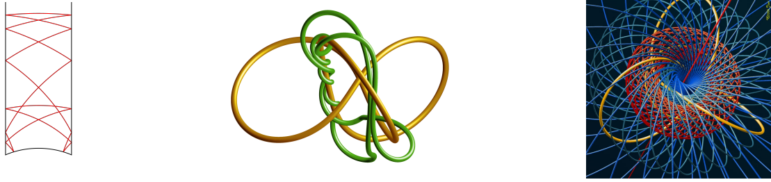
A modular geodesic in \mathbb{M} , lifted as a modular knot in \mathbb{U} , Seifert fibration \mathbb{U} \rightarrow \mathbb{M} . Images produced by Constantin Kogler and Jos Leys with Étienne Ghys .
