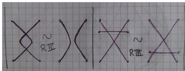
Figure 4.4: Regular homotopies in \mathbb{M} : Reidemeister moves II & III, singular moves.
