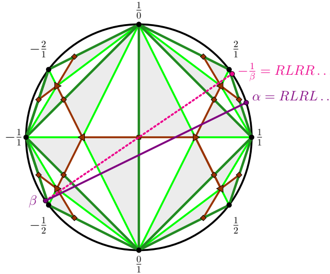
Figure 2.6: Geodesic of \mathbb{P}(\mathbb{H}) intersecting the gliders of \Delta'_2 according to a sequence \dots \mathfrak{t}^{-2} \mathfrak{s}^{-1} \mathfrak{t}^{-1} \mathfrak{s}^{-1} \mid \mathfrak{t}^{+1} \mathfrak{s}^{-1} \mathfrak{t}^{-1} \mathfrak{s}^{-1} \dots , the separation marks the intersection with the base glider.
