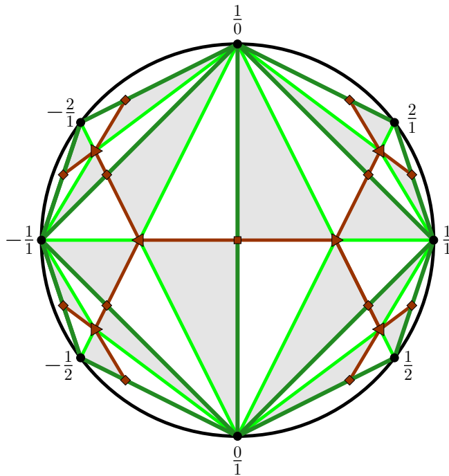
Figure 3.1: The hyperbolic plane \mathbb{HP} is triangulated by \Delta'_2 . The union of a grey triangle and a white triangle forms a fundamental domain under the action of \Gamma .
