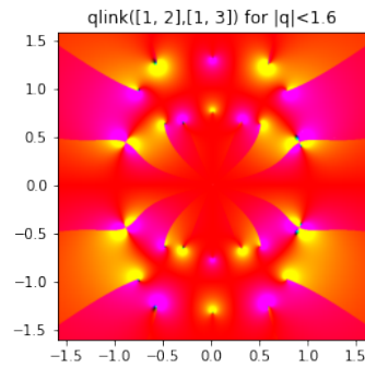
Graphs of L_q(A, B) for complex q .
