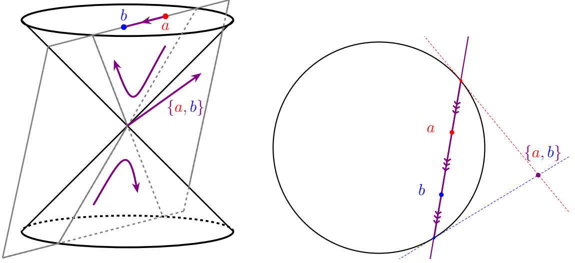
Figure 1.9: The one parameter group generated by \{a, b\} , which is contained in \text{Span}(\mathbf{1}, \{a, b\}) , acts by translation along the line (a, b) .
