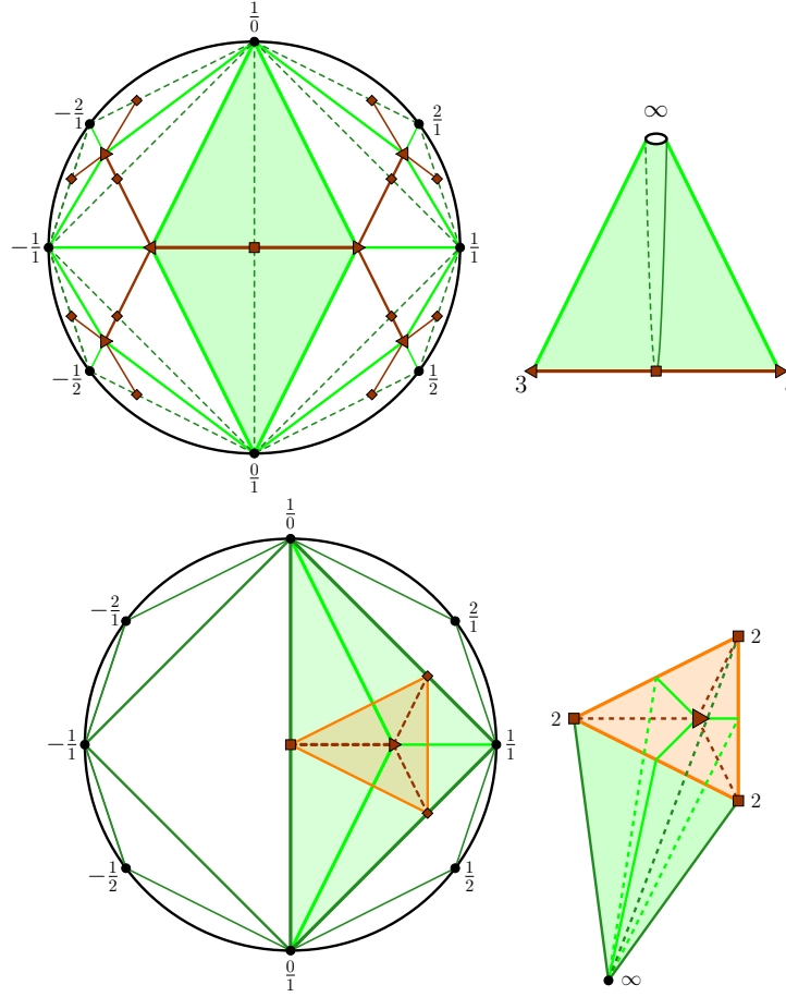
Figure 3.10: Tilings of \mathbb{H}^2 under the kernels of \Gamma \rightarrow \mathbb{Z}/2 and \Gamma \rightarrow \mathbb{Z}/3 . The quotient orbifolds are the only two covers of \mathbb{M} with conical singularities.
