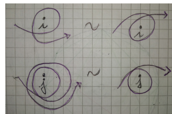
Figure 4.4: Regular homotopies in \mathbb{M} : Reidemeister moves II & III, singular moves.
