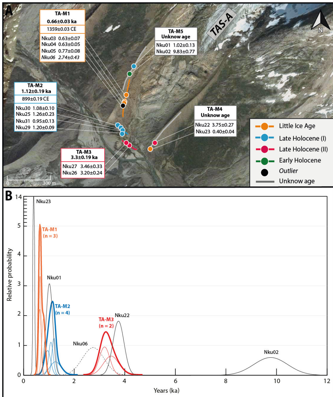
Figure 69 : A. Chronology of glacial advances dated from five moraines of TAS-A glacier in the Tasilap valley. B. Camel plot displaying individual (thin lines), summed (thick lines) and rejected (dashed black lines) ^{10}\text{Be} CRE ages collected. Distributions were calculated with free-MATLAB code from Greg Balco at the University at Washington Cosmogenic Isotope Lab available from http://depts.washington.edu/cosmolab/pubs/gb_pubs/camelplot.m . The number of glacial advance stages recorded during the Late Holocene are noted (I), (II), (III) as an informal indication in Figs 68–71.
