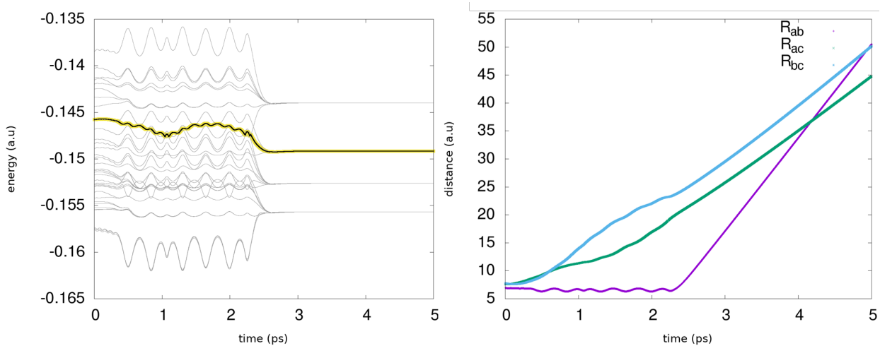
Figure 7.3: An example of a long-lived trajectory in \text{Ar}_3^* where R_{ab} , R_{bc} and R_{ac} in right side figure are the interatomic distances.
