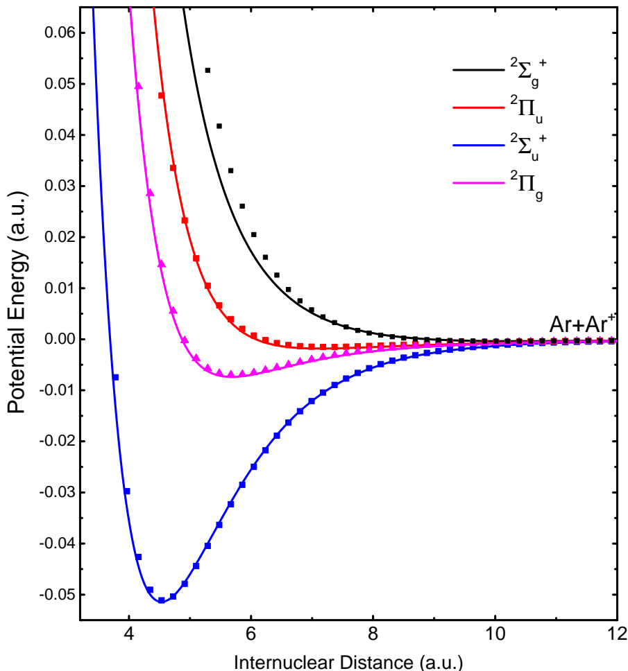
Figure 2.5: CCSD(T) PECs of \text{Ar}_2^+ plot from MOLCAS using aug-cc-pV5Z basis (Lines) and Mastalerz et al. [89] (Points). The 0 is associated to the ionic dimer dissociation.
