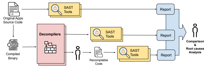
Figure 4.1: Summary of the Experiment Pipelines
