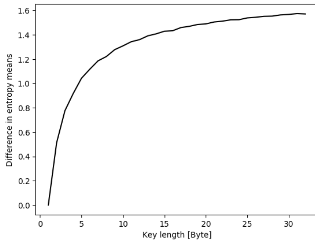
Figure 3.2: Encrypted .text section – difference in entropy means
