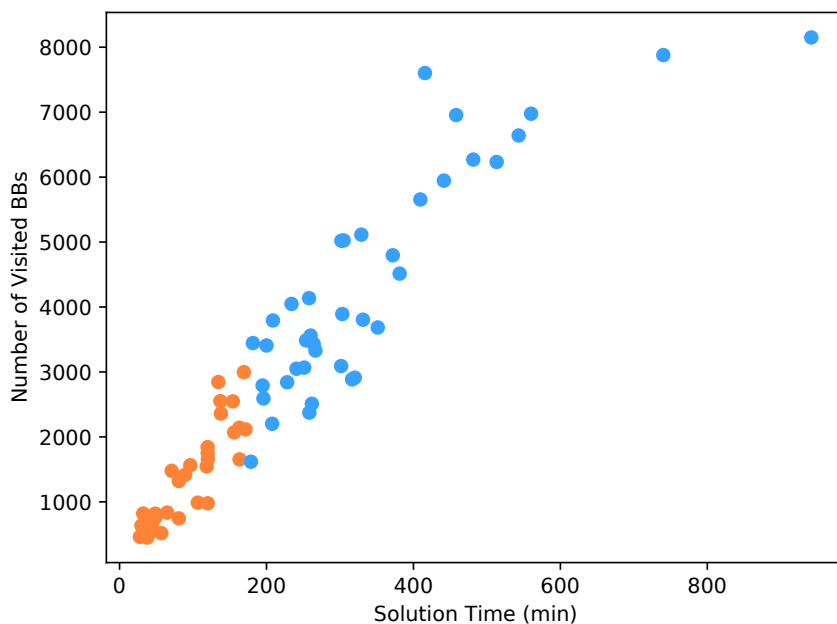
Figure 5.10: Solution time w.r.t. number of visited BBs.
