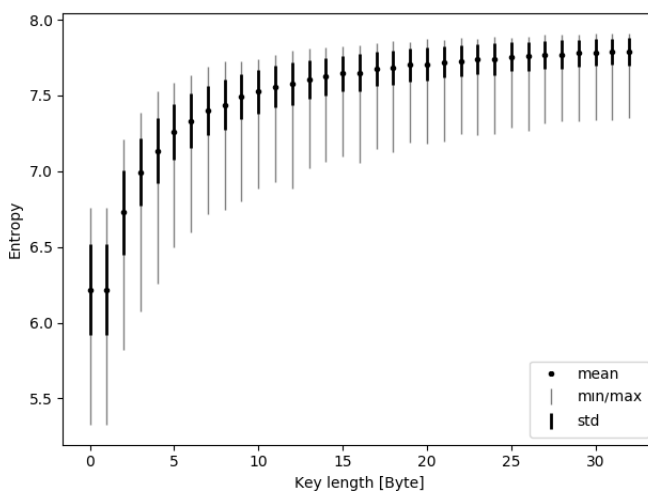
Figure 3.1: .text section entropy w.r.t. XOR encryption
