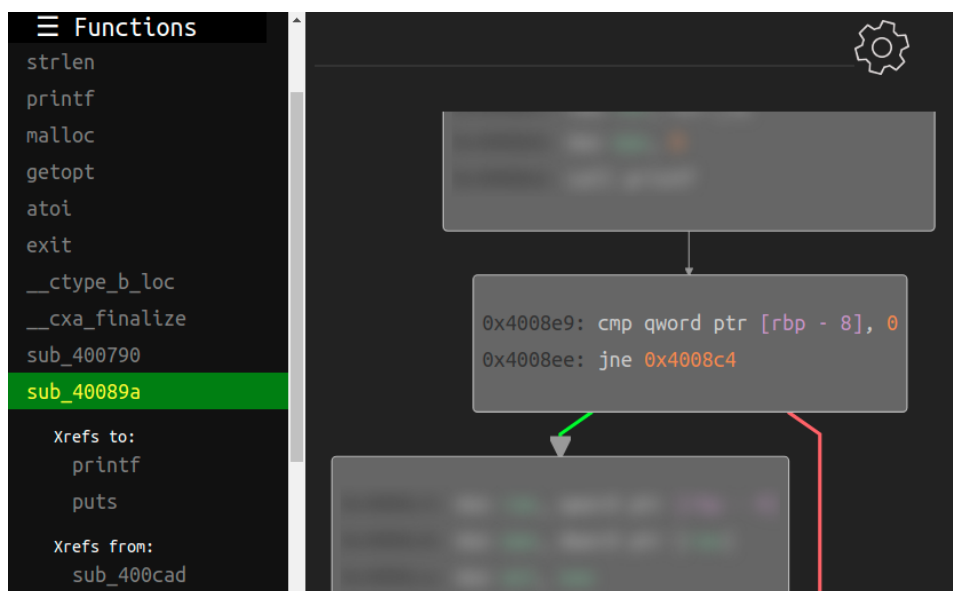
Figure 5.1: Part of the UI of our reverse engineering framework in the code navigation mode showing on the left the functions' list and on the right the CFG of the selected function
