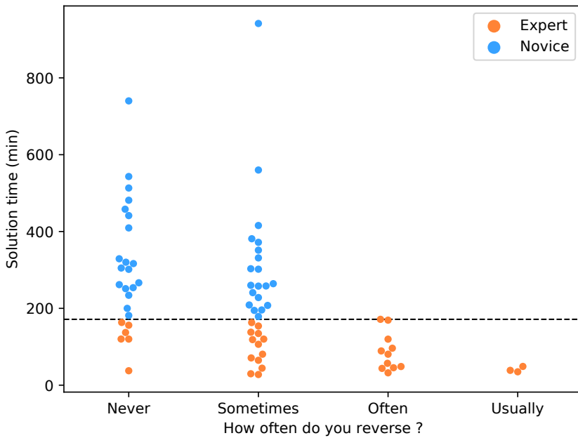
Figure 5.4: Relationships between how often the subject reverse binaries and the total time spent to solve the exercises.
