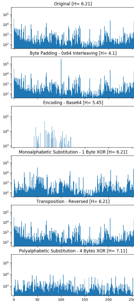
Figure 3.3: Byte Frequency Distribution w.r.t. Schemes
