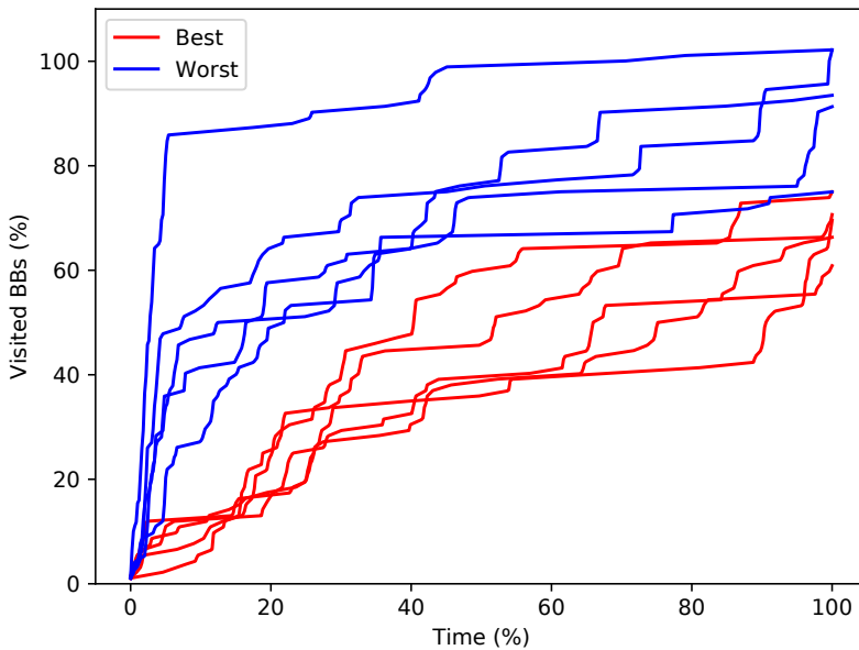
Figure 5.8: Progression of Top5 and Bottom5 experts in the second challenge.
