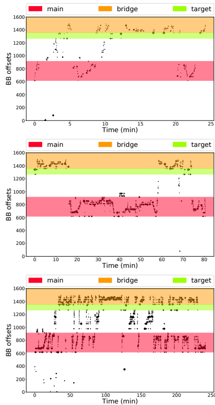
Figure 5.5: Three distinct RE sessions of Test 1 showing the time spent on each basic block during the session
