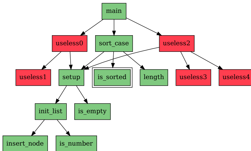
Figure 5.3: Call Graph of Test 2
