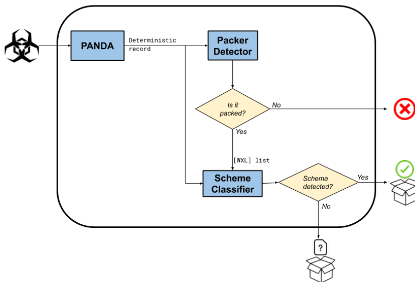
Figure 3.5: Architecture of our analysis tools
