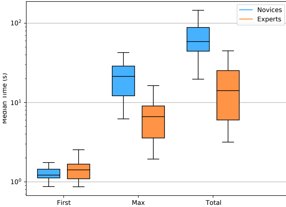
Figure 5.9: Comparison of the distribution of T_{First} , T_{Max} , and T_{Total} time among the users in the two groups.
