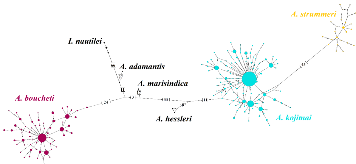
Figure 24: Haplotype network of 722 individuals of Alviniconcha spp for Cox1 partial mitochondrial sequence. Circles represent individual haplotypes, while circle size is proportional to haplotype frequency. The numbers on the branches indicate the number of mutations between haplotypes. Purple: A. boucheti ; Turquoise: A. kojimai and Yellow: A. strummeri .
