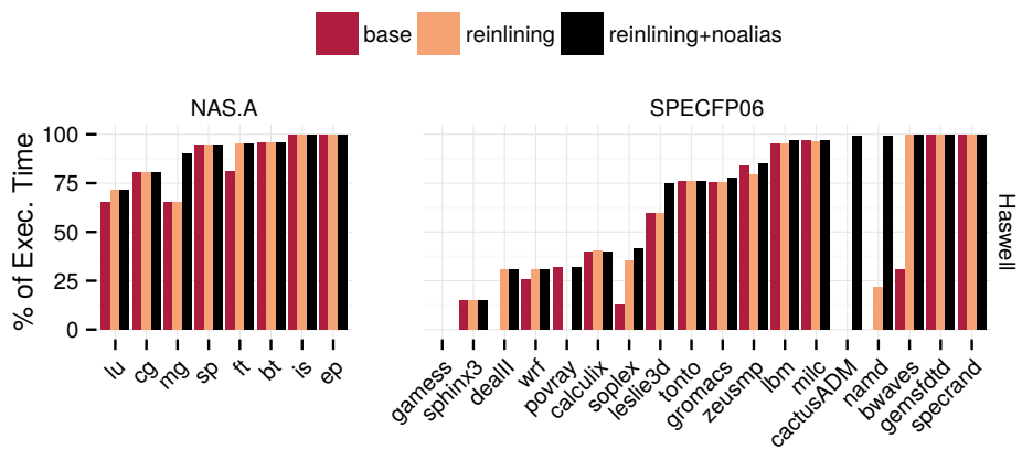
Figure 2.12: Percentage of execution time accurately replayed (error < 15%) on the NAS and SPEC FP benchmarks with different replay configurations. ReInlining and explicitly marking cloned variables as NoAlias improve replay accuracy in eleven benchmarks.
