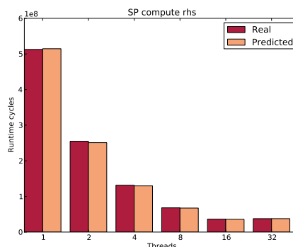
Figure 2.13: Real vs. PCERE execution time predictions on Sandy Bridge for the SP compute rhs codelet
