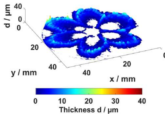
Figure 91: Thickness of the liquid film formed on a piston surface as measured by laser-induced fluorescence imaging (LIF). Image taken at 300 CAD BTDC, injection of liquid fuel at 200 bar at 360 CAD BTDC [109].
