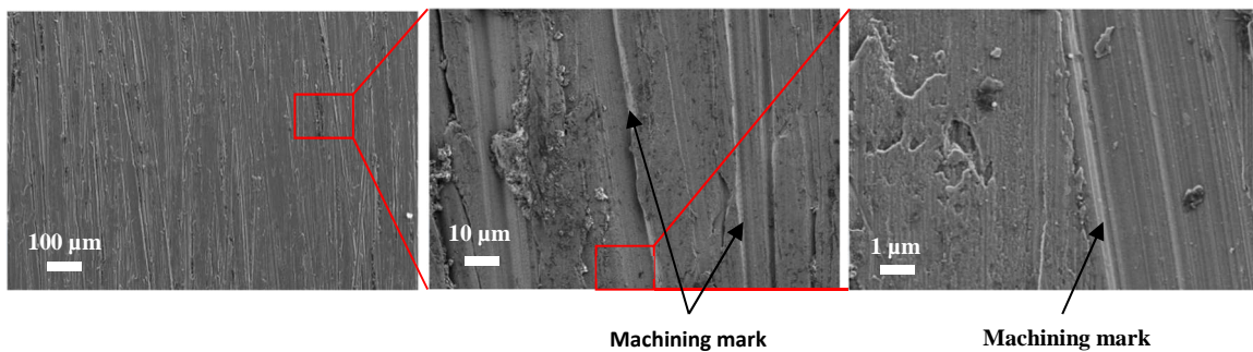
Figure 69: SEM images of the surface of a deposit-free piston.
