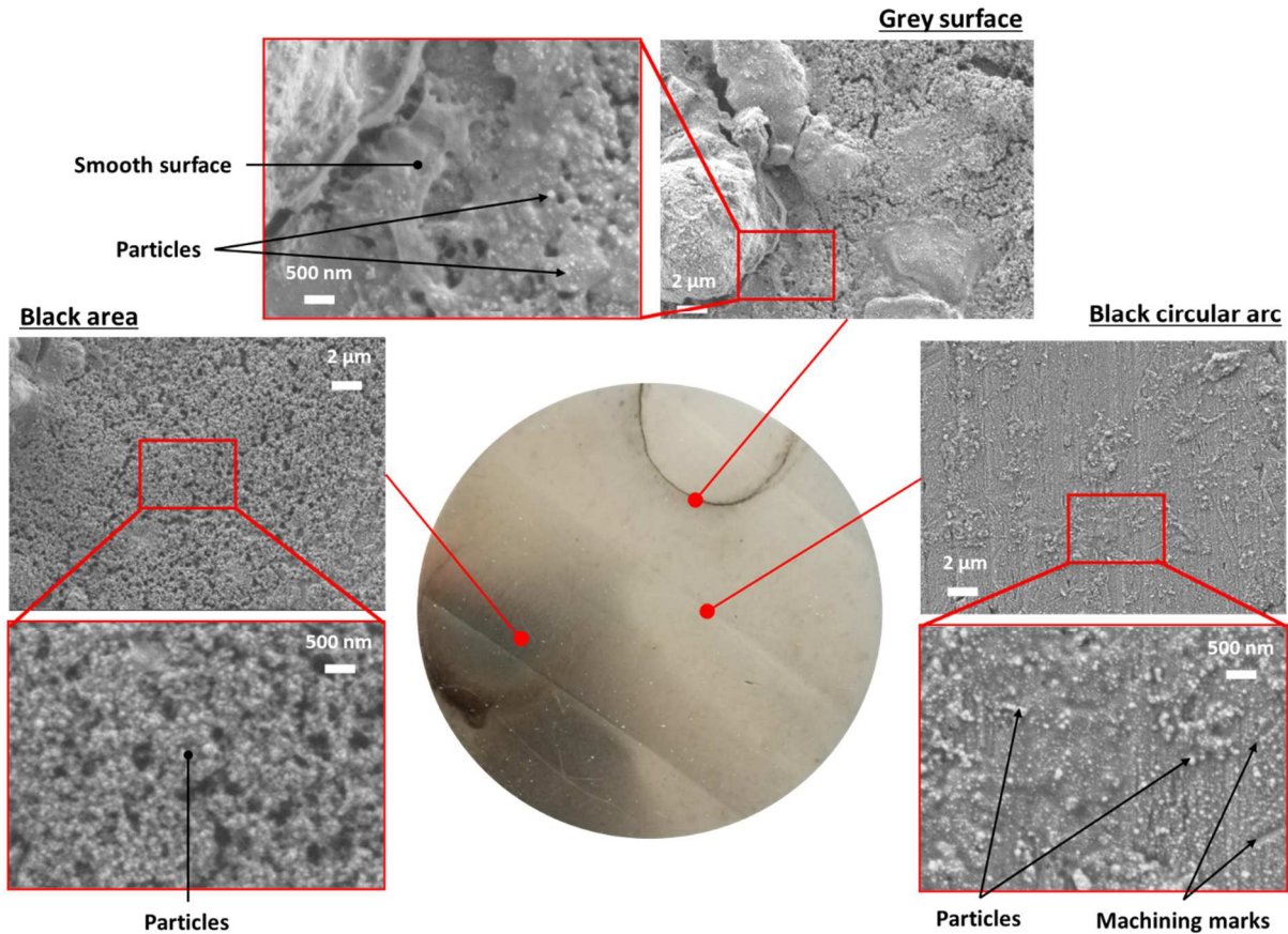
Figure 70: Macroscopic observations by SEM-EDS of the experiment 7 standard injection case.
