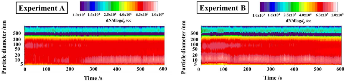
Figure 115: Temporal variation of the soot particle-size distribution in the exhaust for experiments A and B.
