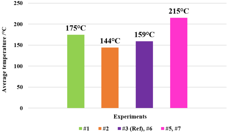
Figure 120: Average piston temperatures for the various warm-start experiments.
