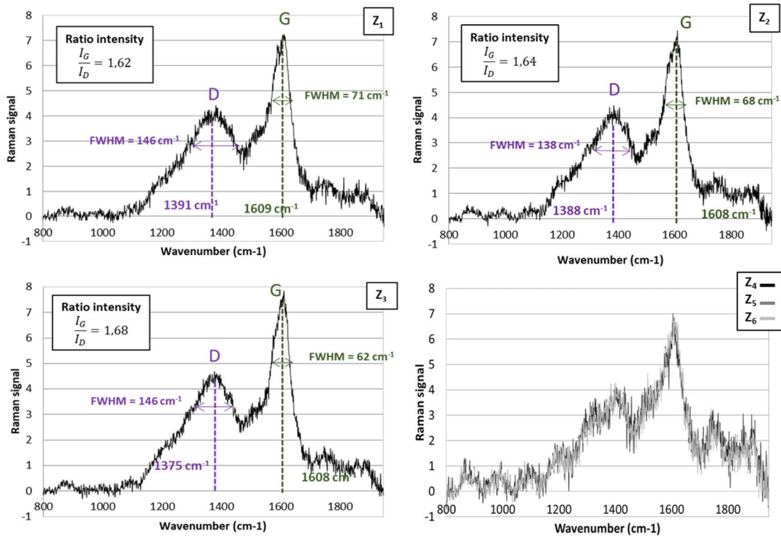
Figure 76 : Raman signal of zones Z_{1-6} for piston deposits from early injection experiment.
