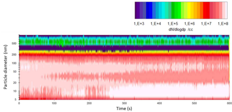
Figure 57: Contour plot of the soot particle-size distribution of the experiment 2.
