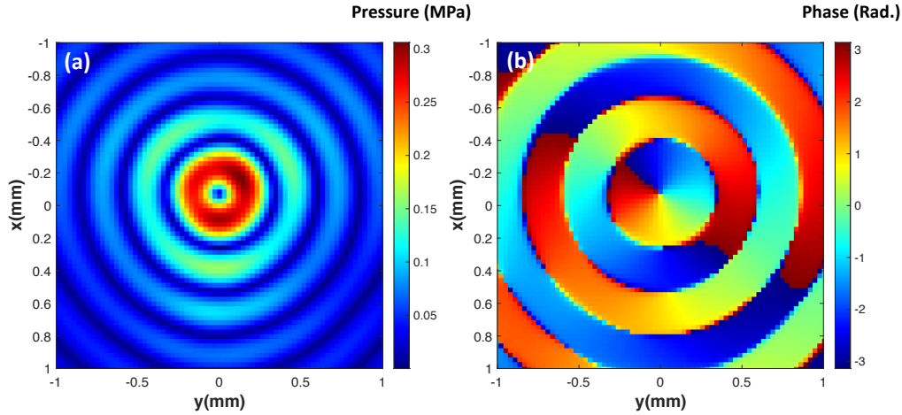
Figure 3.7: Pressure in the focal plane (12 mm above the electrodes) for the LF 3D tweezers with a 1 mm thickness wafer: (a) Amplitude (in MPa), (b) phase (in Radian).
