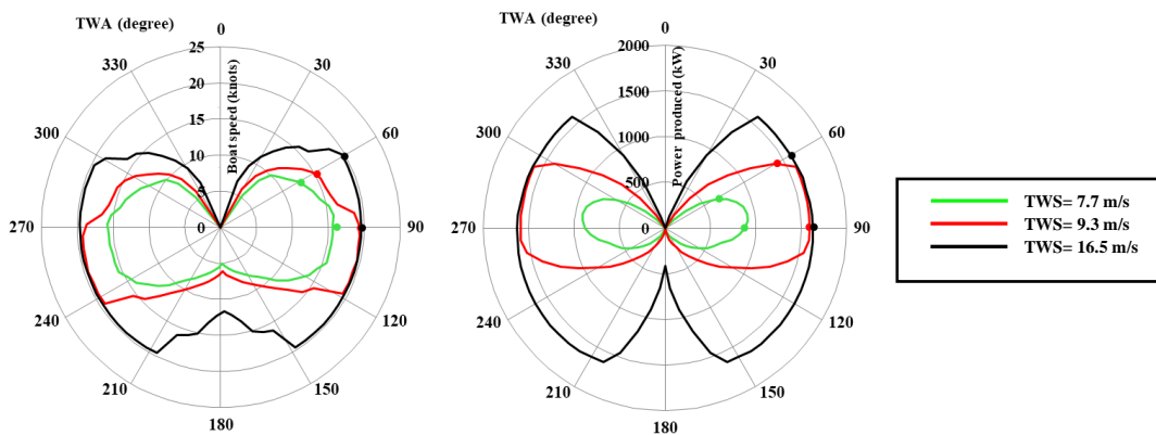
Figure 31 Example of 1.6 MW catamaran boat speed (left) and power production (right) polars
