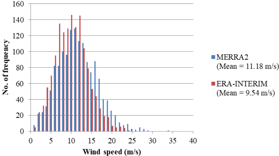
Figure 36 Wind distributions for MERRA2 and ERA-INTERIM dataset for year 2017
