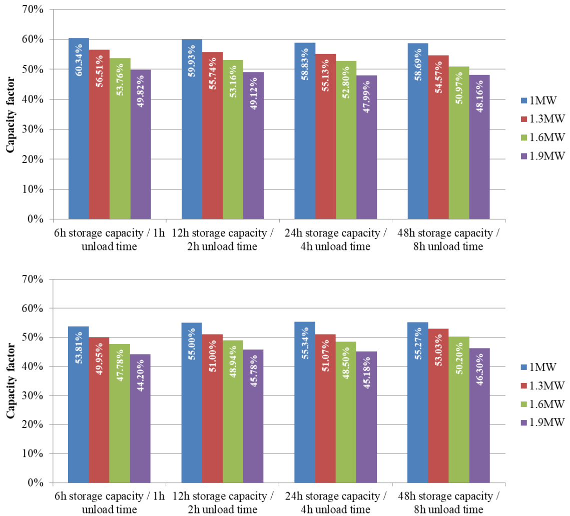
Figure A2- 5 Average capacity factor for 1MW, 1.3MW, 1.6MW and 1.9MW energy ship in (top) Saint-Pierre-et-Miquelon and (below) Ile de Sein for 3 years (2015, 2016, 2017)
