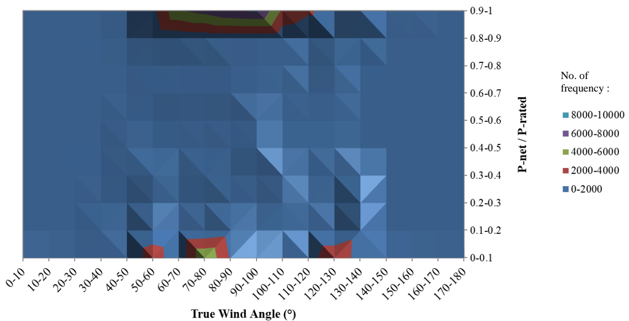
Figure 54 Frequency of true wind angle (°) in response to produced energy over rated power of the 1.6 MW energy ship at Saint-Pierre-et-Miquelon
