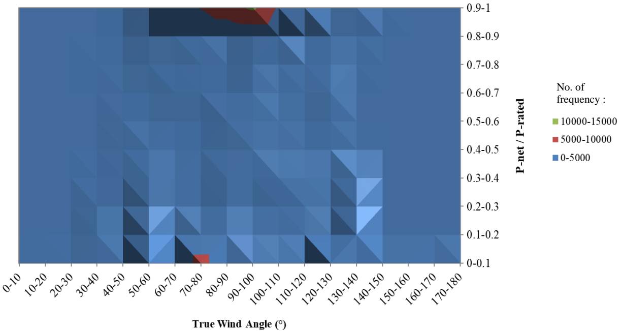
Figure 62 Frequency of true wind angle ( ^{\circ} ) and power production of the 1.6 MW energy ship at Ile de Sein
