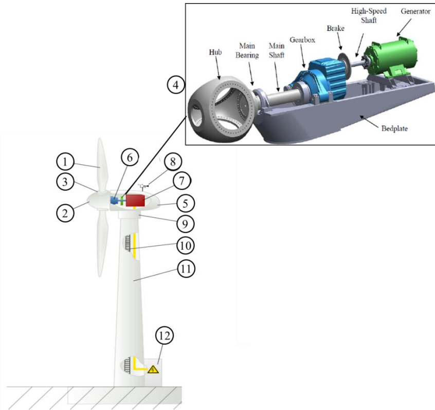
Figure 15 Wind turbine components (Source: [49])
