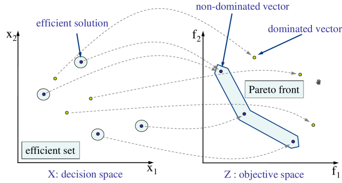
Figure 2-7: Bi-objective representation where f_1, f_2 are the objectives to minimize, and x_1, x_2 are two variables characterizing the solutions.
