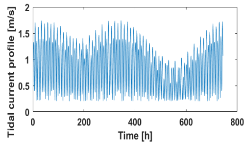
Figure II-23. Monthly tidal current profile for December, 2001.
