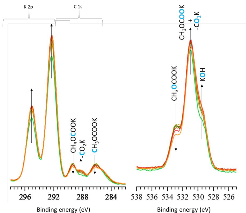
Fig. S3 Evolution of the K 2p-C 1s (left) and O 1s (right) XPS core spectra of the \text{CH}_3\text{OCO}_2\text{K} compound under the X-ray beam (from green to orange). Up and down arrows indicate an increase or decrease in component intensity, respectively. \text{K}_2\text{C}_2\text{O}_4/\text{RCO}_2\text{K} ( -\text{CO}_2\text{K} components) and KOH impurities increased during acquisition.
