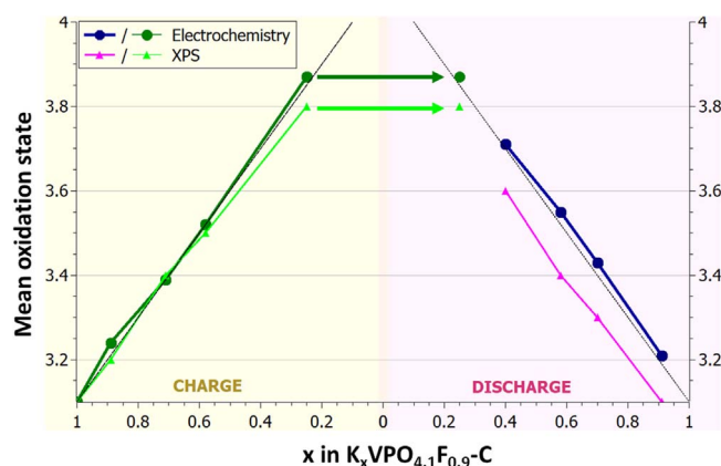
Figure 2. Vanadium mean oxidation state (DO) of \text{KVPO}_4\text{F}_{0.9}\text{O}_{0.1}\text{C} , as the K content changed during the 3rd cycle, determined from the charge/discharge capacity on one side and from the analysis of the XPS spectra on the other side. Grey lines represent the theoretical DO based on the \text{KVPO}_4\text{F}_{0.9}\text{O}_{0.1}\text{C} formula.
