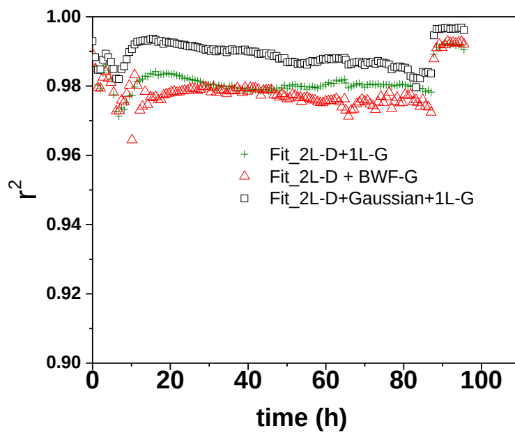
Figure S5. : r^2 values compared for different fit models
