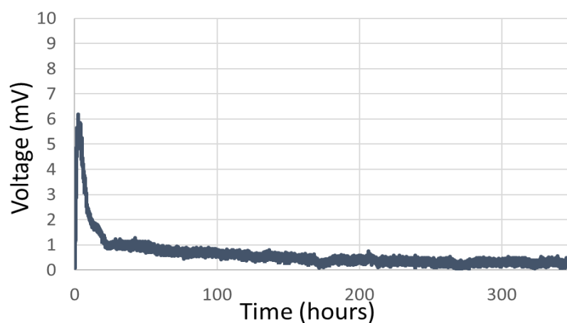
Fig. S3. Typical open circuit voltage profile of a symmetric K//K cell using 0.8M KPF 6 in a mixture of EC:DEC (in volume) as electrolyte.
