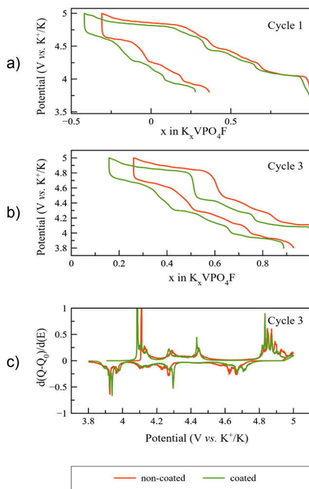
Fig. S4. Voltage profiles of the 1 st (a) and 3 rd (b) cycles obtained for the K//KVPF (red curves) and K//KVPF-C (green curves) electrochemical cells at C/5 (26 mA.g -1 , i.e. the exchange of 1K + in 5 hours) and 20°C. As observed, x is significantly higher than 1 during the first cycle. Thus, XPS analyses were performed during the 3 rd cycle, where much lower electrolyte degradation occurs, as observed. (c) Differential capacity versus V during the 3 rd cycle.
