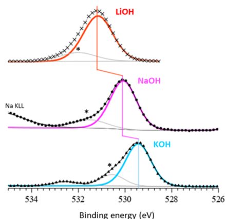
Figure 4. O 1s XPS core-level spectra of LiOH (red cross), NaOH (pink point), and KOH (blue triangle). Intensities were maximized for better comparison. An asterisk indicates that these peaks are attributed to \text{M}_2\text{CO}_3 impurities.
