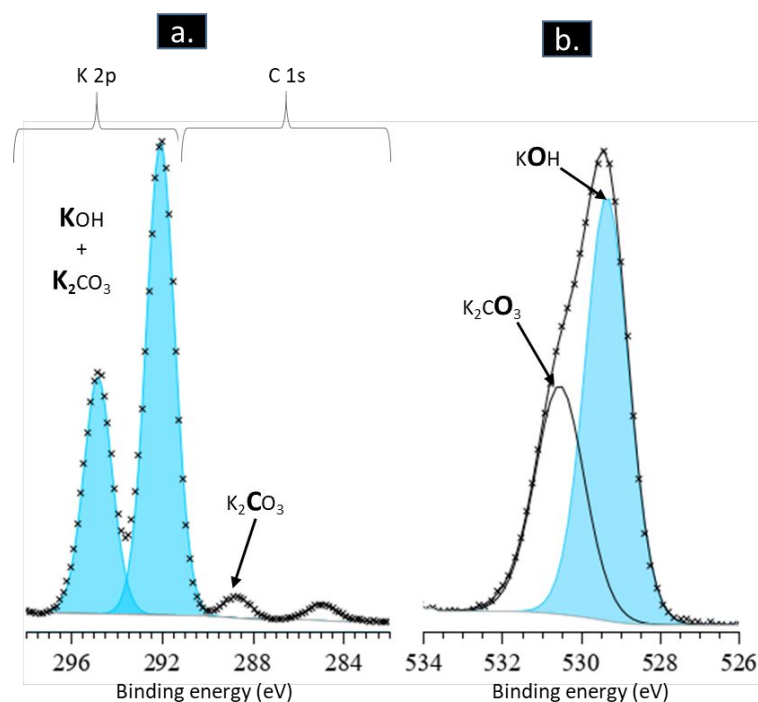
Fig. S2 a) K 2p-C 1s and b) O 1s XPS core level spectra of a \text{K}_2\text{CO}_3 -KOH sample. This sample was prepared by aging a KOH pellet (KOH powder grinded in a mortar then compressed) for 1 week under air so that \text{K}_2\text{CO}_3 was formed at its reactive surface.
