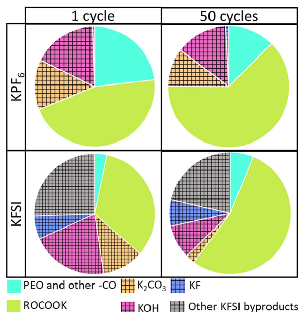
Fig. 3. SEI composition as derived from XPS quantification of CNF electrodes recovered from CNF/K cells after 1 and 50 cycles, using 0.8M of either KFSI or KPF 6 in EC:DEC as electrolyte. Striped/plain areas highlight inorganic/organic species.
