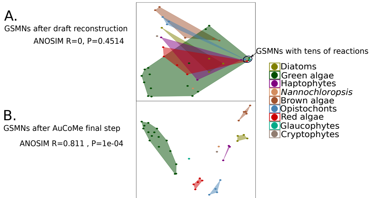
Figure 3.8 – MDS showing the metabolic distance between GSMNs of the different groups of organisms in the algal dataset. Subplot A represents the GSMN distances after the draft reconstruction step, and subplot B shows the GSMN distances after the final step of AuCoMe. The metabolic distances were computed using a presence-absence matrix of reactions among species in the algal dataset. ANOSIM values indicate the difference in variance between different groups. Close to 0, it is not possible to differentiate the group and close to 1, it is possible to differentiate the group. MDS and ANOSIM were computed using the vegan package (Oksanen et al. 2020).
