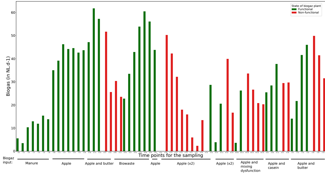
Figure 4.6 – Measure of the biogas production in the biogas reactor experiment (Awhangbo et al. 2020). The abscissa axis corresponds to the time points of the measure of the biogas. Below the abscissa axis, the inputs of the biogas reactor over time are described. The ordinate axis indicates the biogas production in NL.d-1, Normal litre per day, a unit used to measure the gas production on a normal temperature and pressure (in our case 20° C and 1 standard atmosphere), as the volume taken by the same quantity of gas can change according to these two parameters. The bars in green correspond to time points where the biogas reactor was labelled as functional, and the bars in red correspond to time points where the biogas reactor was described as non-functional.
