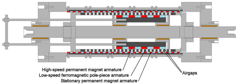
Fig. I-31 The tubular linear magnetic gear prototype cross-section presented in [77].
