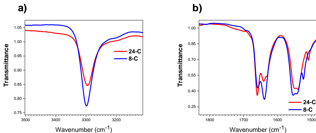
Figure IV. 13 FTIR powder spectra of 8-C and 24-C .
