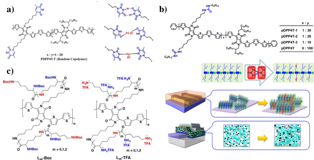
Figure 1. 47 a) Chemical Structure of PDPP4T-T ; Thymine groups are randomly connected to the conjugated backbone and the illustration of T-T Intermolecular H-bonding and the coordination with Pd(II) and Hg(II). [285] b) Chemical Structures of pDPP4T-1 , pDPP4T-2 , pDPP4T-3 , and pDPP4T , and illustration of the design rationale for the incorporation of urea groups in the side chains of conjugated D-A polymers. [287] c) Chemical structures of DPP polymers containing lysine residues. [288]
