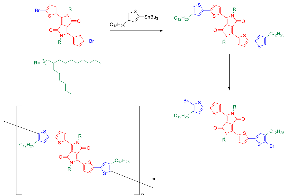
Scheme IV. 1 Summarized synthetic approach of an alkylated bithiophene DPP polymer derivative.
