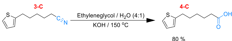
Scheme IV. 9 Optimized conditions for the hydrolysis of the nitrile into a carboxylic acid.
