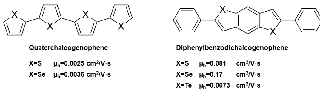
Figure I. 10 Influence of heteroatom replacement in mobility values for two different molecules used for organic semiconductors. Mobilities were measured for vacuum deposited films of the materials. *Adapted. [60]
