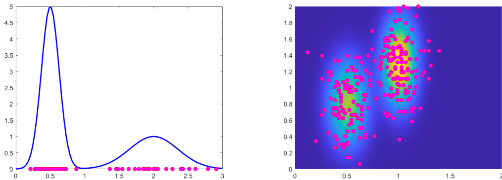
Figure 5.13: On the left, we represent the one-dimensional acceptance-rejection method applied to f(x) = 5e^{-30(x-0.5)^2} + e^{-4(x-2)^2} with x \in (0, 3) and the counter limit M = 100 . On the right, a two-dimensional example with f(x, y) = 5e^{-30(x-0.5)^2 - 4(y-0.8)^2} + 7e^{-40(x-1)^2 - 4(y-1.3)^2} with x, y \in (0, 2) and the counter limit M = 250 .
