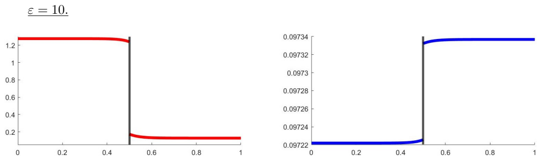
Figure 4.22: With \varepsilon = 10 , the slow reaction is not prevailing significantly on the diffusion (since increasing the value of \varepsilon , reactions converge to zero). The permeability of the membrane promotes dissipation but a slope nearby the interface is still observed.
