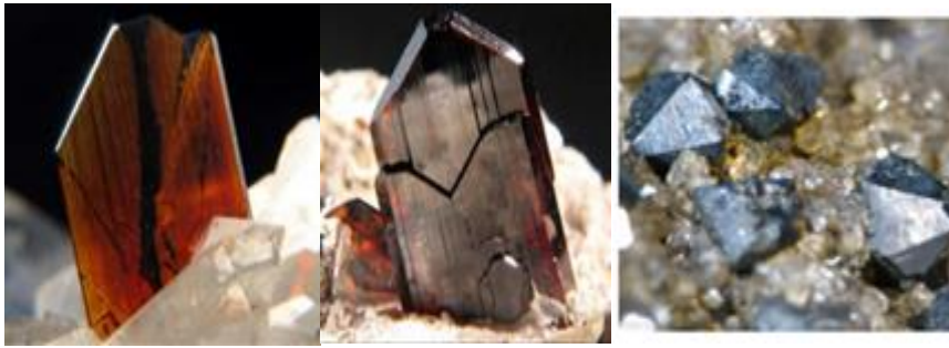
Fig.I.6 La brookite [18, 29]
