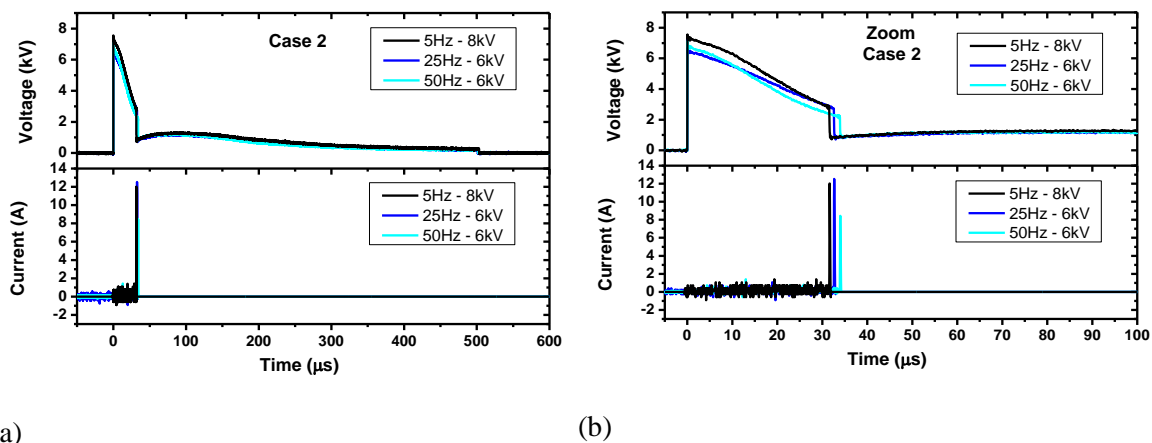
Figure A 22 Electrical waveforms of pin-to-pin discharge for case 2 generated in water for different frequencies and voltages , V = 200 \text{ mL} , \Delta t = 500 \text{ } \mu\text{s} , 2 \text{ mm} of gap, and \sigma = 200 \text{ } \mu\text{S/cm} ; (a) Voltage and Current signals and (b) a zoom of these signals.
