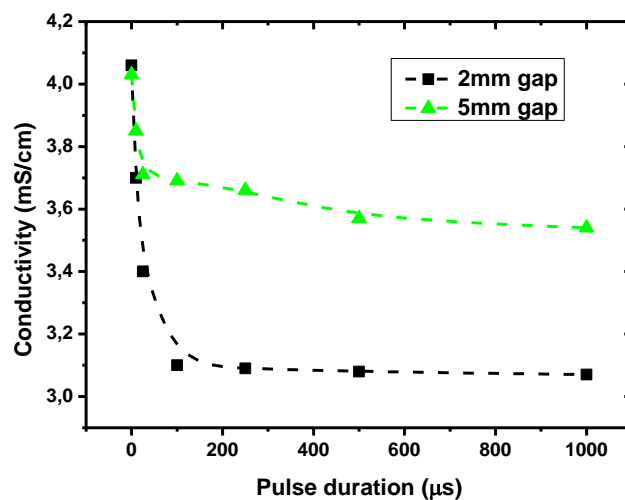
Figure 6.16 Final solution conductivity versus pulse duration for 2 and 5 mm gap of a pin-to-pin discharge obtained in Cr(VI) solution (47 mg/L, \sigma=4 mS/cm, pH=2.4) U = 9 kV, V = 100 mL, f = 50 Hz, electrodes length = 0 \pm 10 \mu\text{m}
