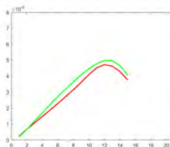
(d) Central velocities (NT in green, PSM in red): NT proliferation rate equal to 0 at t = 12 hours.
