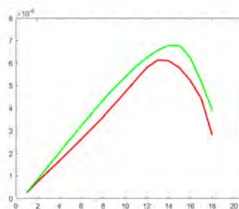
(b) Central velocities (NT in green, PSM in red): Injection rates in the PSM and NT are equal to 0 at t = 12 hours.
