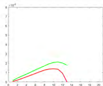
(c) Central velocities (NT in green, PSM in red): PSM proliferation rate equal to 0 at t = 12 hours.
