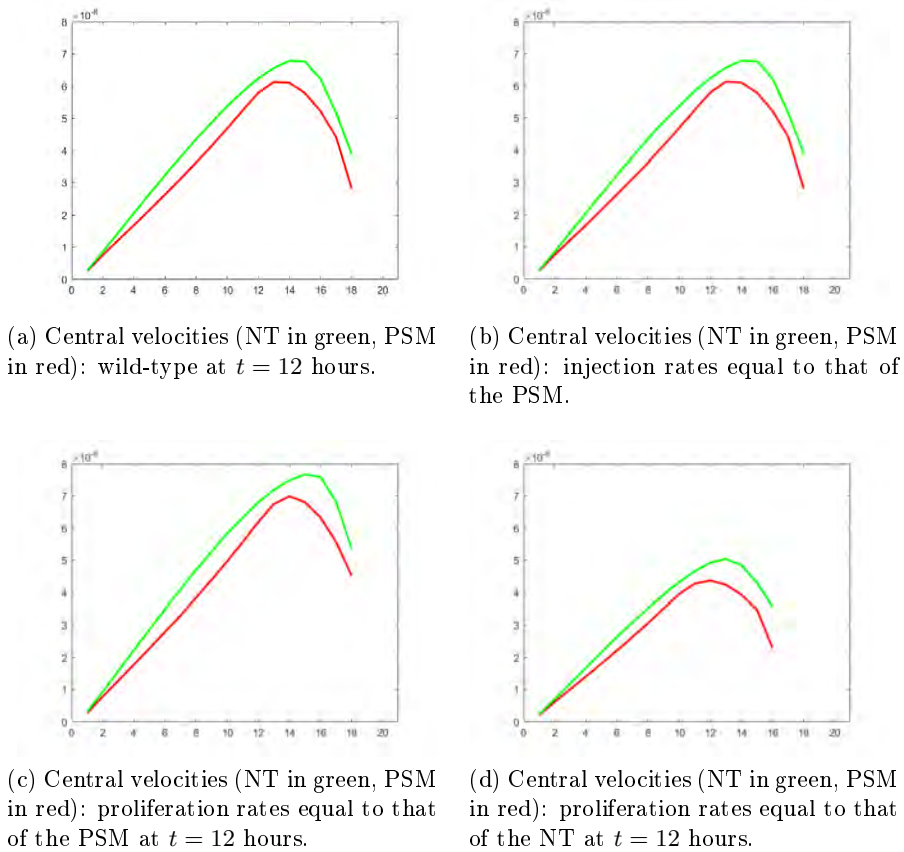
Figure 5.7 – Central velocities of the NT in green and the PSM in red at t = 12 hours in the wild-type case (Panel (a)), when injection rates are equal to that of the PSM (Panel (b)), when proliferation rates are equal to that of the PSM (Panel (c)) and when proliferation rates are equal to that of the NT (Panel (d)). The y -axis is in units m/s (value of the velocity), the x -axis represents the mesh cells along the antero-posterior axis.
