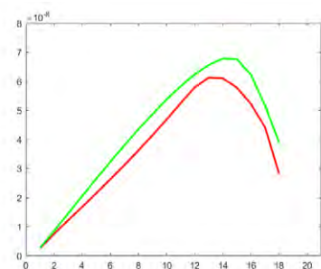
(a) Central velocities (NT in green, PSM in red): wild-type at t = 12 hours.
