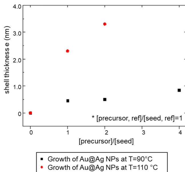
Figure 2.16. Temperature and silver precursor concentration effects on the final size of Au@Ag NPs.
