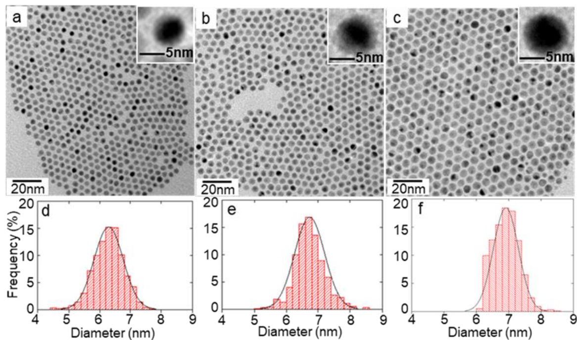
Figure 2.8. Representative TEM images of Au 5nm (PC)@Ag NPs obtained from different seed concentrations (a) C_{seed} , (b) C_{seed}/2 and (c) C_{seed}/4 where C_{seed} = 1.4 \mu\text{mol L}^{-1} and (d, e, f) the corresponding histogram. In inset: TEM images at higher magnification.
