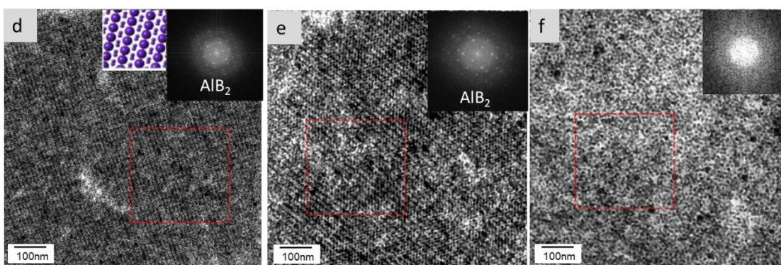
Figure 4. 5. TEM images of binary nanoparticle superlattices formed from \gamma\text{-Fe}_2\text{O}_3 and Au NPs with effective size ratio of (1) \gamma_{\text{eff}} = 0.45 and (2) 0.48 formed after evaporation of different nature of solvent (a) and (d) toluene, (b) and (e) hexane and (c) and (f) chloroform. Insets indicate selected area FFT analysis. Representation of unit cell of each BNSL structure corresponding to TEM image is presented as an inset (left side from FFT diagram).
