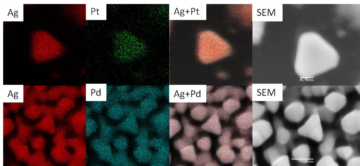
Figure 2.30. Typical SEM images of 3D superlattices made of Ag_{12nm}@Pt D_{CS}=13.7 nm and Ag_{12nm}@Pd D_{CS}=13.0 nm and cartography of each atom using EDX analysis.
