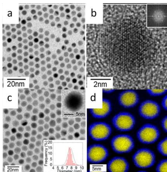
Figure 2.13. (a) typical TEM image of the corresponding Au_{5nm}(SC)@Ag NPs with a silver thickness e=0.2 nm obtained for C_{Ag^+} = 0.825 mmol L^{-1} and T=90^{\circ}C (b) HRTEM image of one corresponding single NP. (c) typical TEM image of Au_{5nm}(SC)@Ag core-shell NPs with a silver thickness e=0.85 nm obtained for C_{Ag^+} = 1.65 mmol L^{-1} and T=80^{\circ}C and (d) corresponding EELS map showing the Au core (yellow) and the silver shell (blue).
