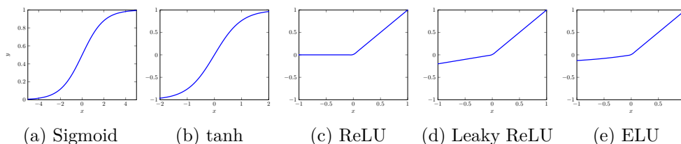
Figure 1.6: Familiar activation functions.
