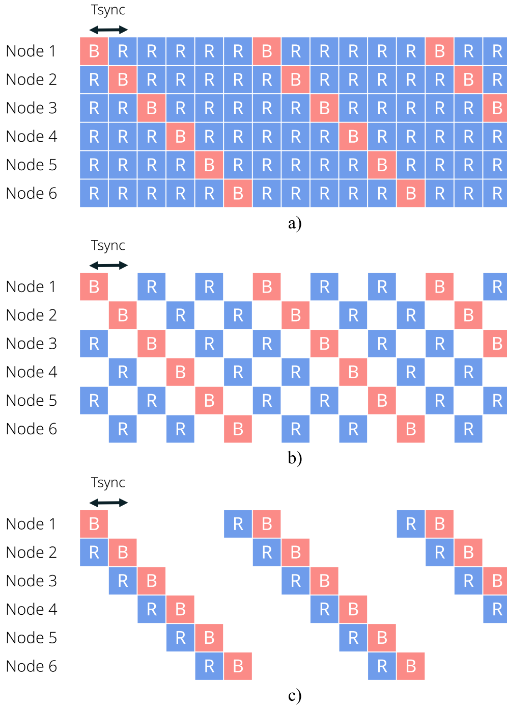
Figure 4.5 – a) Sleep mode schedule presented in the previous section for a network of 6 nodes. All the nodes wake-up every Tsync to receive or send a beacon and synchronize the network. b) Energy reduction attempt for the proposed sleep mode. In this case we create two synchronization loops, so node 1, 3 and 5 will lose synchronization with nodes 2, 4, and 6. c) Another energy reduction example which produces the synchronization swing phenomenon.
