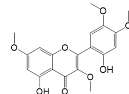
2,5-dihydroxy-3,4',5',7-tetramethoxyflavone
