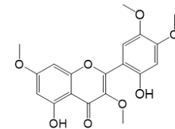
2,5-dihydroxy-3,4',5',7-tetramethoxyflavone
