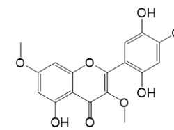
2',5,5'-trihydroxy-3,4,7-trimethoxyflavone
