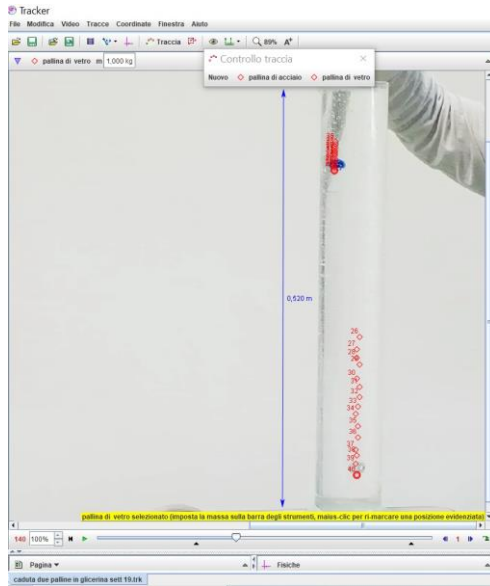
Fig. 4.8. An example of using Tracker software to calculate the terminal speed. The position of the little ball was marked every 4 cs. Source: my experiment image.
