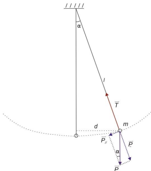
Fig. 3.4 Forces acting on a pendulum. Source: my own representation.
