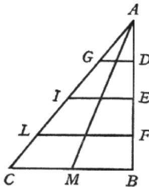
Fig. 2. Galileo showed that if a body falls freely along smooth planes inclined at any angle whatsoever, but of the same height, the speeds with which it reaches the bottom are the same and that the travel times are proportional to the lengths of the planes . Galilei [1638], 1890-1909, vol. VIII, p. 216. Source: Bibliothèque nationale de France / gallica.bnf.fr.
