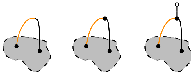
Figure 2.1: The bijection between half-edge rooted (1,3)-valent maps (left) and vertex-rooted open rooted trivalent maps (right) obtained by first subdividing the root-containing edge of the former (middle step) before finally adding a new vertex.
