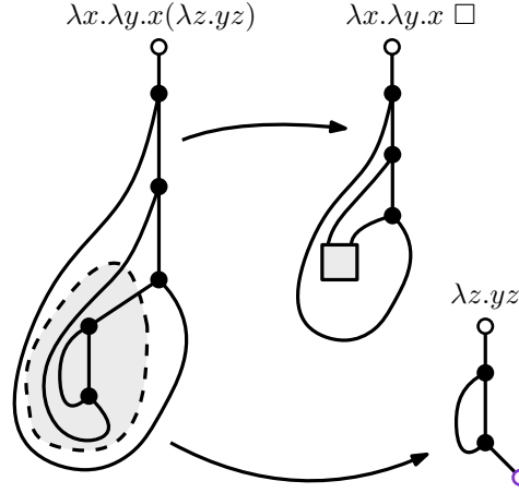
Figure 2.5: A decomposition of t = \lambda x.\lambda y.x(\lambda z.yz) , as c[u] for c = \lambda x.\lambda y.x \square and u = \lambda z.yz , corresponding to a 2-cut in the map \tau^{-1}(t) .
