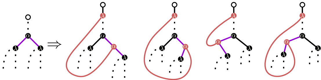
Figure 4.35: Possible forms of an abstraction falling under Case 2 of Theorem 4.4.21
