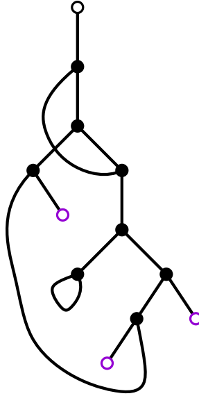
Figure 4.8: Example of a vertex-rooted (1,3) -valent map corresponding to the underlying map of the linear term \lambda x. \lambda y. (((a((yc)b))(\lambda z.z))x) . Since the 1-valent vertices are unlabelled (compare with the open rooted trivalent maps in Figure 2.2 ), the map captures the structure of the \lambda -term up to permutation of the free variables (a, b, c) .
