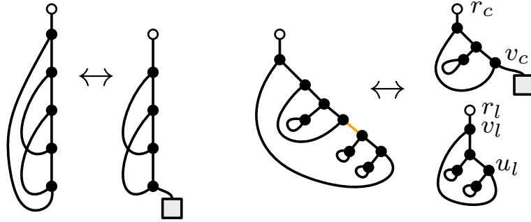
Figure 4.5: Maps corresponding to elements of \dot{\mathcal{T}}_{[0]} and their decompositions. For the subfigure on the left, we have a decomposition of \lambda x.\lambda y.\lambda z.xzy into \lambda y.\lambda z.\square zy , which is of the form \mathcal{Z}^2\mathcal{Q} . For the map on the right we have a decomposition of \lambda x.\lambda y.x(\lambda a.a)(\lambda b.b)y(\lambda c.c) into \lambda y.\square y(\lambda c.c) and \lambda x.x(\lambda a.a)(\lambda b.b) of the form \mathcal{Q}\dot{\mathcal{T}}_{[0]}^\lambda . Vertices in the right subfigure are labelled as in the proof of Lemma 4.2.12 and the internal bridge b is highlighted.
