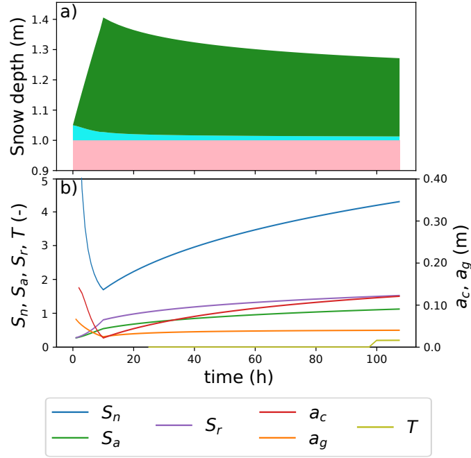
Figure 2.6: Temporal evolution of the snow depth (a) and of the associated stability models (b) during and after a snowfall. The slab (dark green) is composed of new snow with a moderate density (initial value of 100 \text{ kg m}^{-3} ). The weak layer (blue) is composed of very light snow (initial density of 50 \text{ kg m}^{-3} ). The slab and the weak layer evolve with time due to snow settlement. The substratum (pink) is composed of hard snow and do not evolve with time. Legend names refer to models described in Table 2.1.
