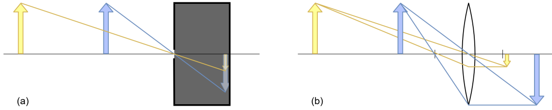
Figure 2.9: (a) A pinhole camera does not need to be focused, because in theory, only one single ray per object point will pass through the aperture—which incidentally makes the image dimmer. (b) On the contrary, more light rays can pass through a lens, which makes the projected image clearer—but incidentally, it introduces a finite depth of field, as the image is focused on a different plane depending on the object distance to the lens.
