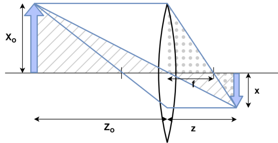
Figure 2.10: Thales’ theorem leads to the thin lens equation. X_O is the object of size, and Z_O its distance to the lens; x is the image size, and z its distance to the lens; and f is the focal length f .
