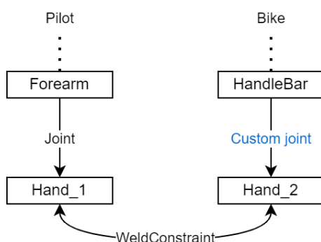
Figure 7.4: The trick used to break the kinematic chain, and constrain it while keeping more degrees of freedom than OpenSim allows. Any custom joint could be used (e.g., a cylindrical joint), and joint limits could be adjusted.
