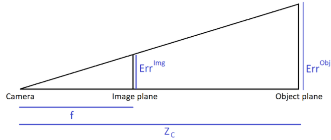
Figure 4.2: The pinhole camera model permits a correspondence between image coordinates and object coordinates. f : focal distance, Z_C : object to camera distance, Err^{img} : error on image plane, Err^{obj} : error on object plane. f and Err^{img} are usually expressed in pixels, while Z_C and Err^{obj} are expressed in meters.
