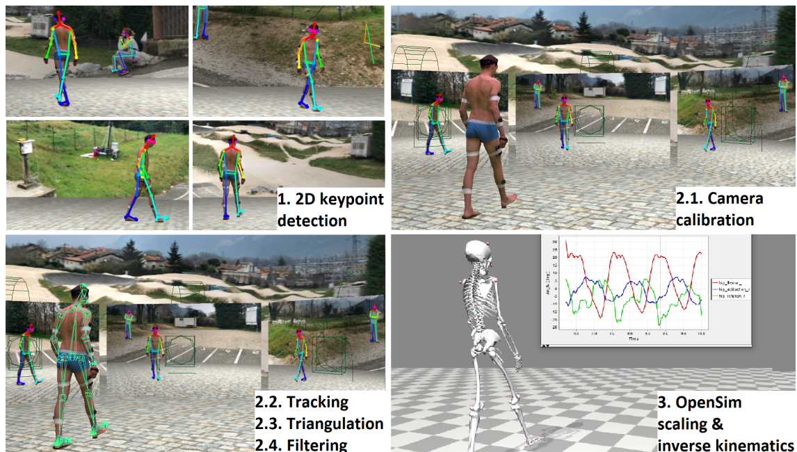
Figure 3.2: Pose2Sim full pipeline: (1) 2D keypoint detection; (2.1) Camera calibration; (2.1-2.4) Tracking of the person of interest, Triangulating of keypoint coordinates; and Filtering; (3) Constraining the 3D coordinates to an individually scaled, physically consistent OpenSim skeletal model.
