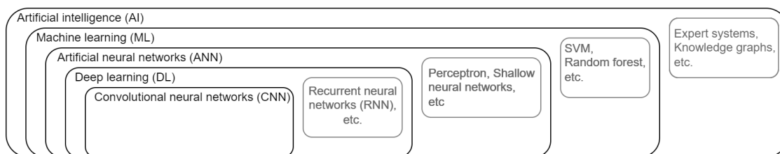
Figure C.12: Inclusion diagram for the concepts of Artificial intelligence, Machine learning, Artificial neural networks, Deep learning, and Convolutional neural networks.
