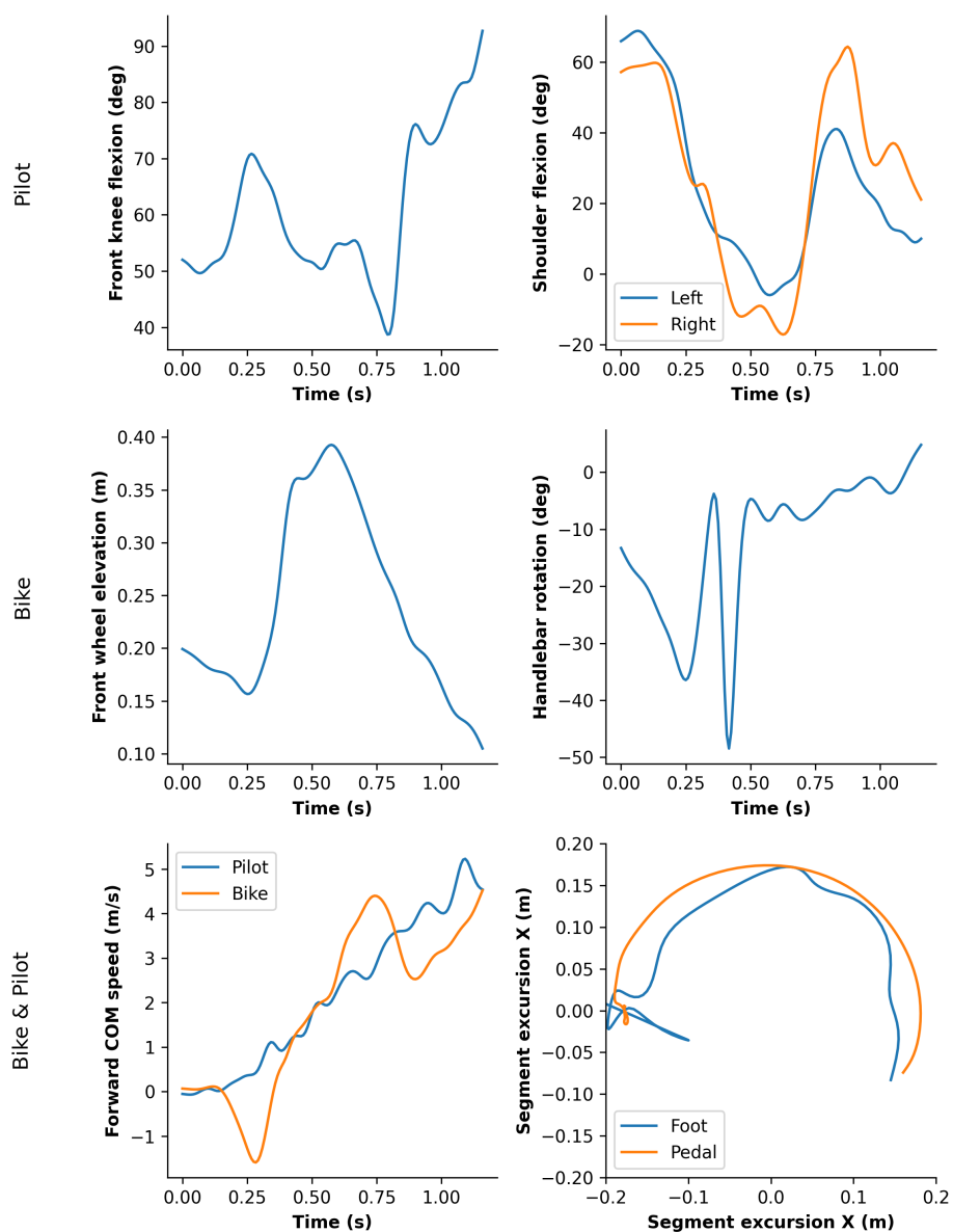
Figure 7.6: Some key performance indicators of the BMX slingshot phase captured with a markerless protocol.
