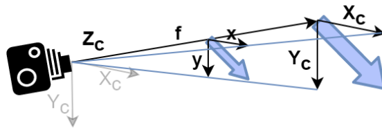
Figure 2.12: The pinhole camera model in 3D.
