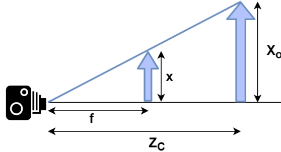
Figure 2.11: The simplified pinhole camera model.
