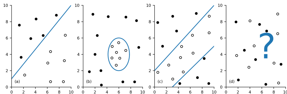
Figure 2.2: Single layer artificial neural networks such as the perceptron can only classify linearly separable data. (a) is linearly separable. (b) is not linearly separable. However, data are contained in an ellipse. The equation of an ellipse is of the form a \times x^2 + b \times y^2 = 1 , so if we transform the feature variables into X = x^2 and Y = y^2 , the data become linearly separable. (c) is equivalent to a fundamental XOR gate, and is not linearly separable, which was part of the reasons for the first AI winter. It can either be solved by combining several layers of artificial neurons, or by complex kernel tricks which map the data from the original space into a higher dimensional space where they become linearly separable. (d) is possibly not separable at all. AI: Artificial Intelligence. XOR: Exclusive OR.
