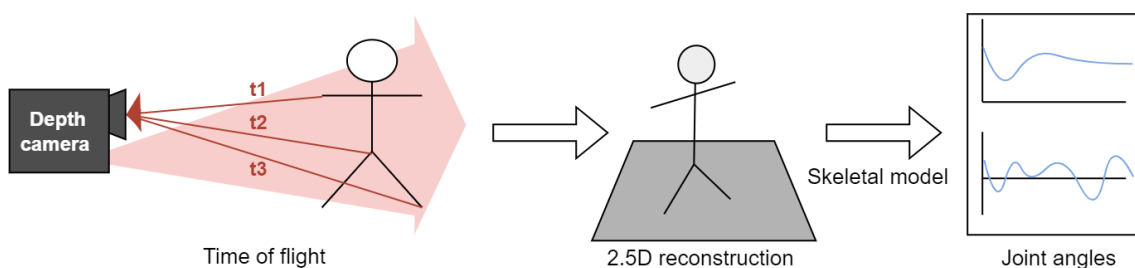
Figure 1.3: A depth-field camera (RGB-D) projects infrared modulated light onto the subject’s body. The time it takes for the light to be reflected to the camera sensor ( time of flight ) depends on distance, and gives access to the depth of the scene. Older RGB-D cameras use structured light rather than time of flight calculations to infer depth.
