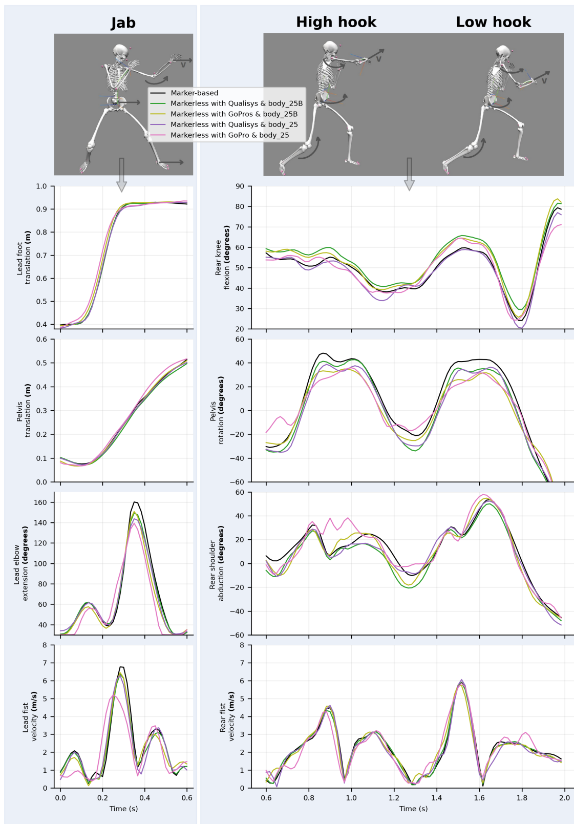
Figure 6.6: A representative trial by one of the athletes. Comparison of selected variables for a sequence of jab, high hook, and low hook in boxing. Waveforms look very similar across all protocols, even though the use of the standard OpenPose body_25 model instead of the experimental body_25B one seems to cause more discrepancy when compared to the reference marker-based analysis.
