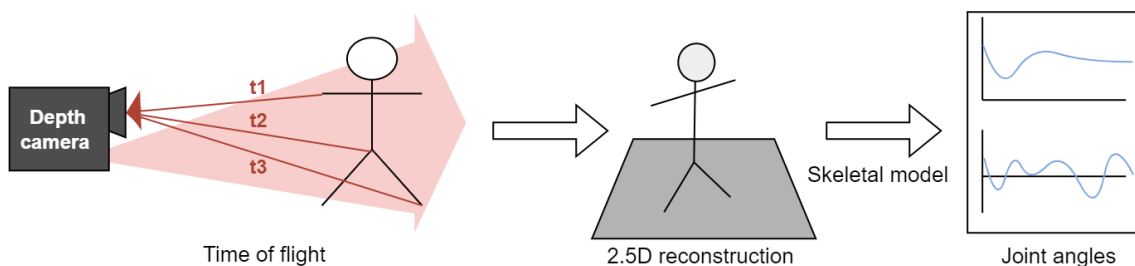
Figure 1.3: A depth-field camera (RGB-D) projects infrared modulated light onto the subject’s body. The time it takes for the light to be reflected to the camera sensor (time of flight) depends on distance, and gives access to the depth of the scene. Older RGB-D cameras use structured light rather than time of flight calculations to infer depth.
