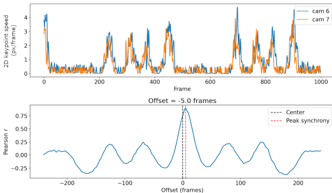
Figure 6.4: Top: 2D keypoint speed comparison between two cameras. Bottom: The offset frame with maximum correlation corresponds to the synchronization offset.
