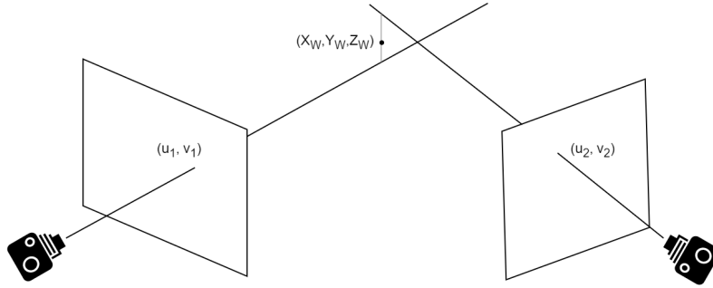
Figure 2.15: The 3D reconstructed point can be approximated as the minimal distance between epipolar lines, which pass by each camera center and 2D detected points.
