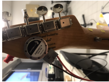
(a) Dayton Audio DAEX19CT-4
