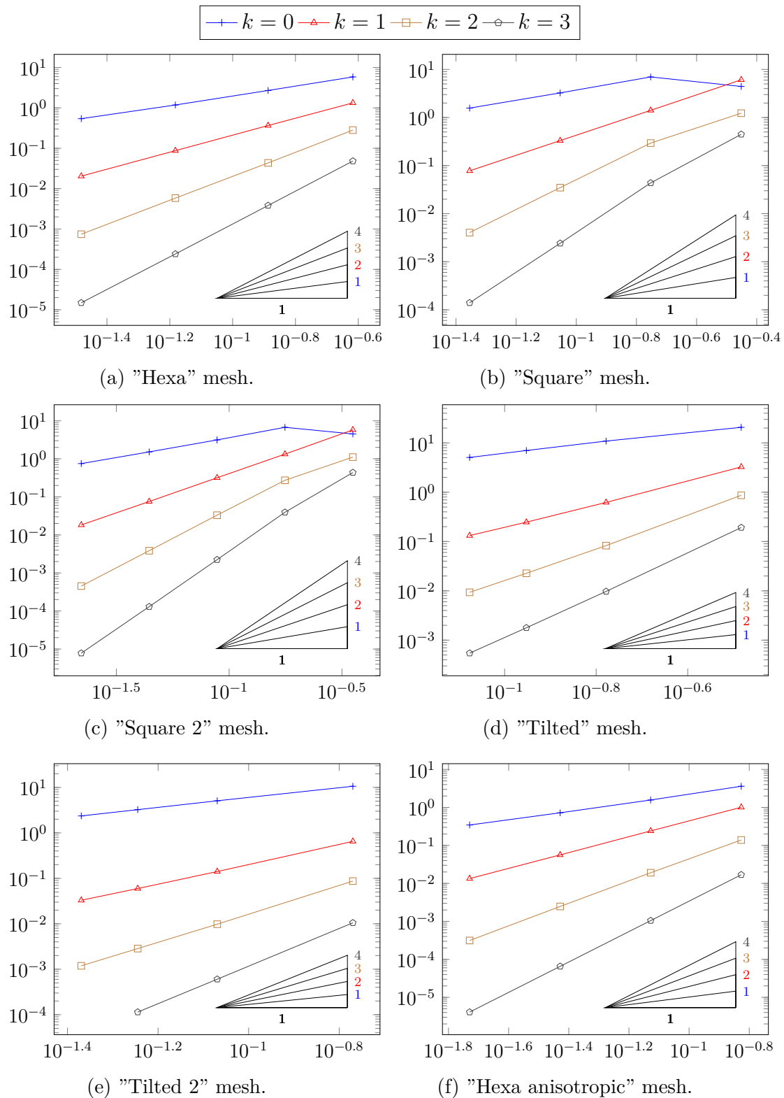
Figure 4.4: Absolute error estimate in discrete norm \|\cdot\|_{\mu,\nabla,1,h} + \|\cdot\|_{L^2,h} vs. mesh size h in 2 dimensions.
