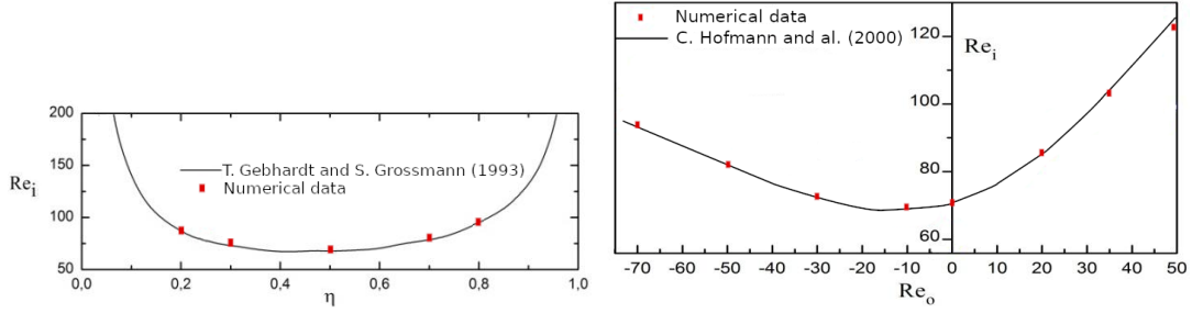
Figure 3.5: Comparison of the critical value of Re_i at Re_o = 0 for various \eta . Figure 3.6: Comparison of the critical value of Re_i at \eta = 0.5 for various Re_o .
