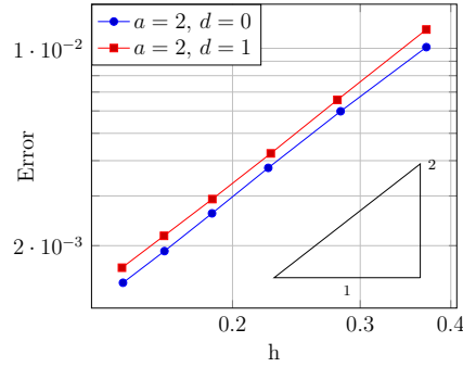
Figure 3.2: Convergence rate of the velocity with relative H(\text{div}) error on a log log scale.
