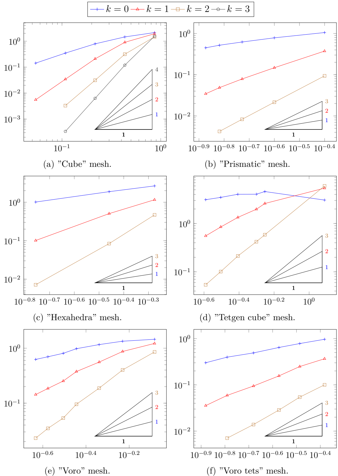
Figure 4.5: Absolute error estimate in discrete norm \|\cdot\|_{\mu,\nabla,1,h} + \|\cdot\|_{L^2,h} vs. mesh size h in 3 dimensions.
