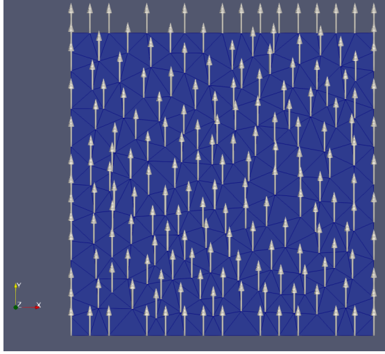
Figure 2.6: Harmonic 1-form on a contractible domain with mixed boundary conditions.
