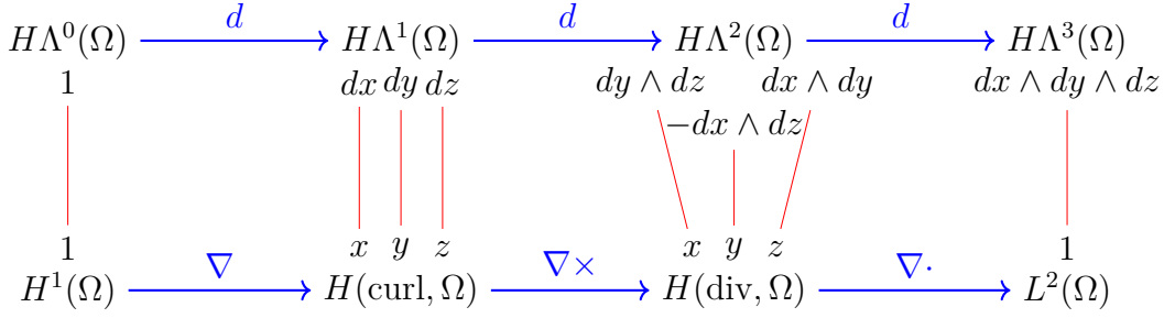
Figure 2.1: Identification between vectors and forms on a domain \Omega \subset \mathbb{R}^3 .
