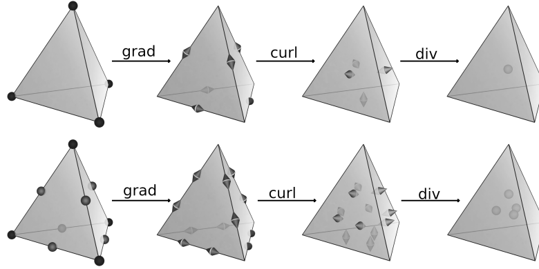
Figure 3.1: Degrees of freedom on reference elements for the polynomial degrees r = 1 and r = 2 .
