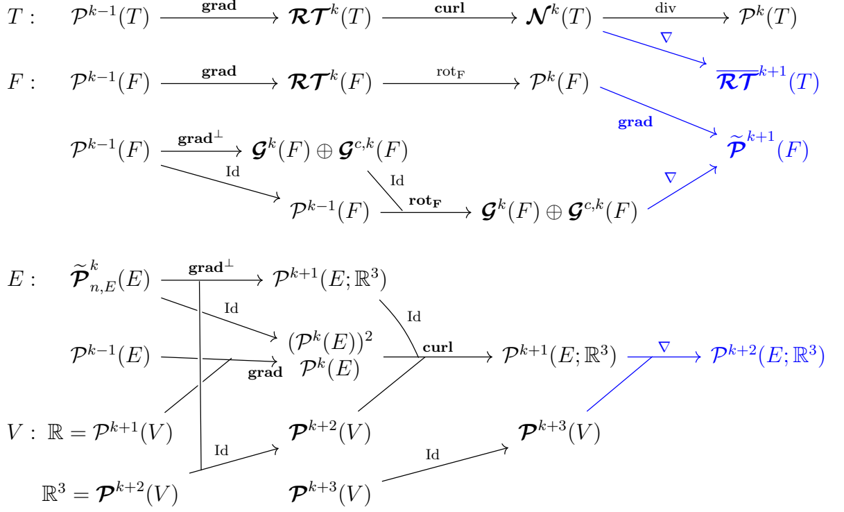
Figure 4.1: Usage of the local degrees of freedom for the discrete differential operators.
