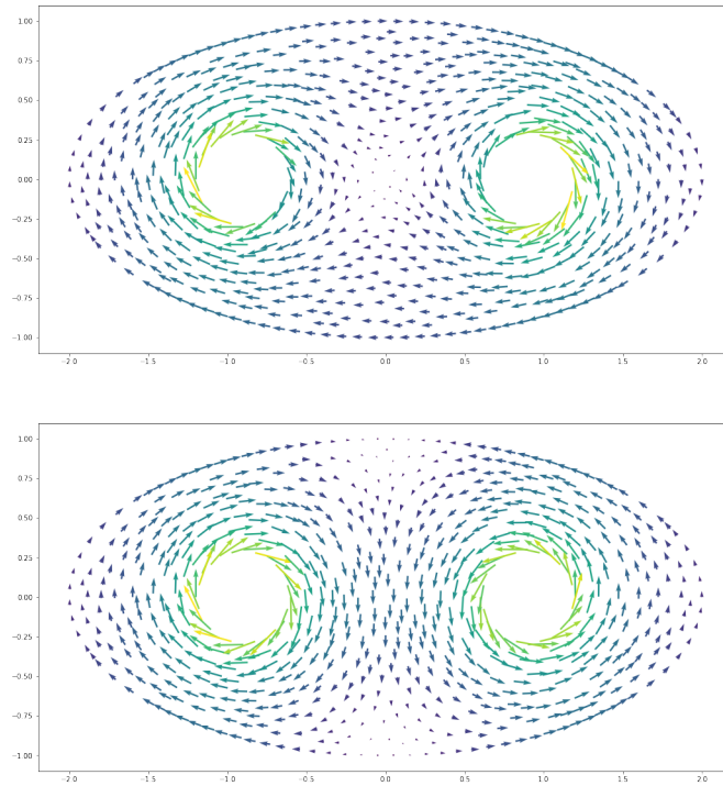
Figure 2.3: Harmonic 1-forms on a surface with two holes.
