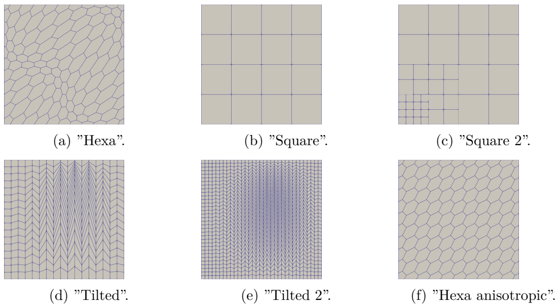
Figure 4.2: Families of meshes used in 3 dimensions, sliced for visualization.
