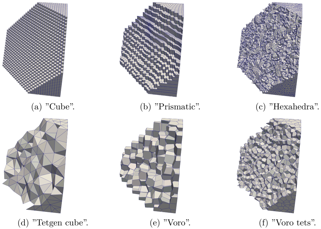
Figure 4.2: Families of meshes used in 3 dimensions, sliced for visualization.
