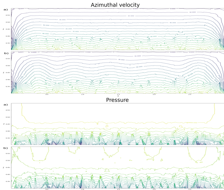
Figure 3.3: Isolines for azimuthal velocity and pressure at \eta = 0.5 , Re_o = 0 , Re_i = 50 (a) and Re_i = 72 (b).
