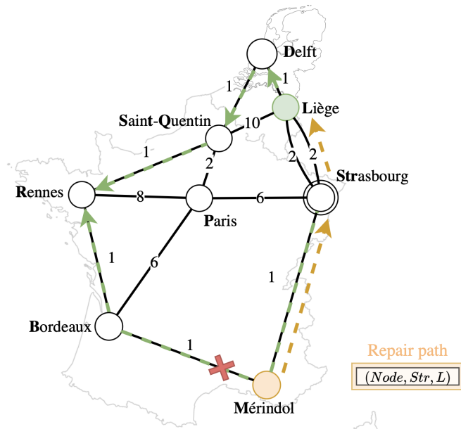
FIGURE 3.1: Example of LFA FRR through Topology Independent LFA (TI-LFA). Mérindol does not have any direct LFA, and thus uses a remote node as a repair node through the use of SR.
