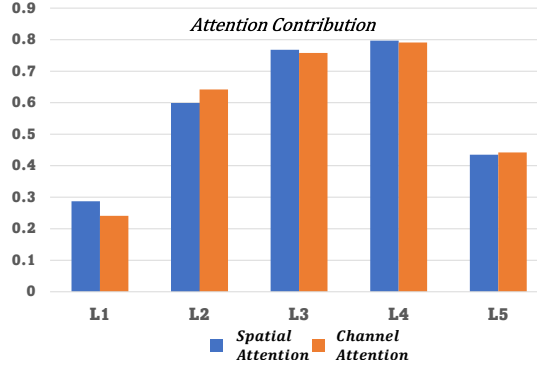
FIGURE 6.8: Attention contribution during feature fusion. L_1, \dots, L_5 stands for the different layers. We realize attention fusion through \alpha \cdot CA + \beta \cdot TSA .
