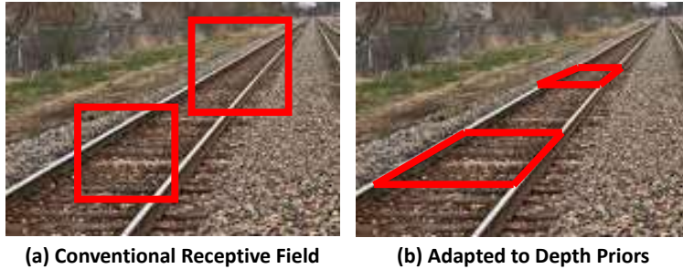
FIGURE 4.1: A sketch of Depth-Adapted Sampling position. We explicitly leverage the depth priors to compute a locally-deformable sampling position, yielding a simple but efficient manner to introduce a global-local attention into CNN.
