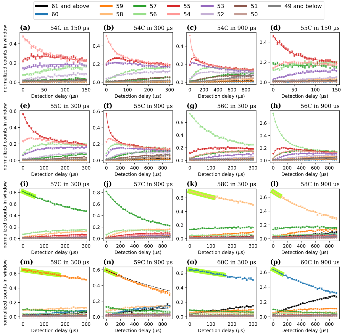
Fig. 4.4 Windowed ion counts from Fig 4.2. The 16 datasets are fitted as a whole with the balanced model as illustrated in Fig. 4.5 (b). The error bars are poissonian errors based on the raw counts of each point. They represent the statistical fluctuations, but are not used to weight the fit. The green highlighted sections are used to obtain the short time exponential t_1 points in Fig. 4.7. In panel (n), the black dashed line gives the long time exponential decay using an optimistic t_1 plotted in Fig. 4.7 (the highest green empty ball).
