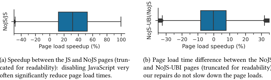
Figure IV.7: Tukey boxplots of the load time differences (measured with the ‘load’ event) when disabling JavaScript and when applying our repairs to the NoJS pages, in our 30,728-page sample
