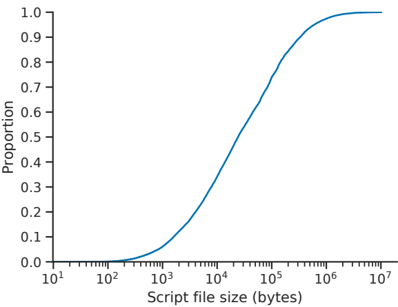
Figure VI.3: File size of external scripts
