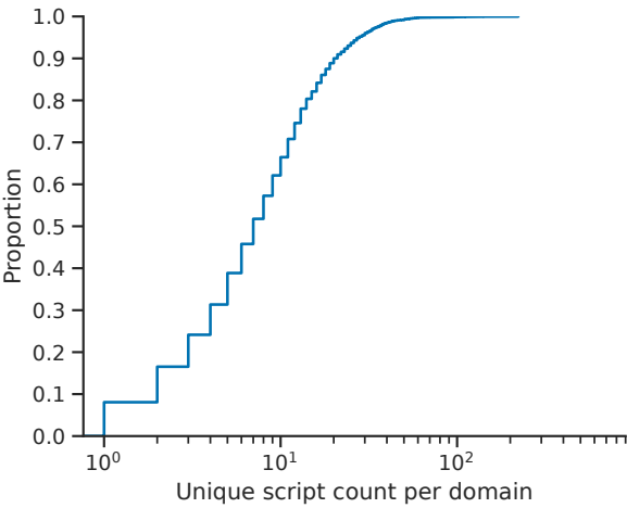
Figure VI.4: Script count per page
