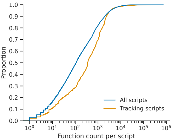
Figure VI.5: Count of functions per script
