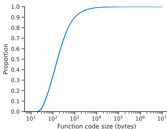
Figure VI.6: Source code size of functions
