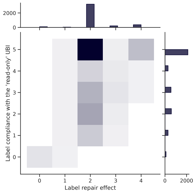
Figure IV.5: Bivariate plot of the manual labeling; the grades are defined in subsubsection IV.3.1.3
